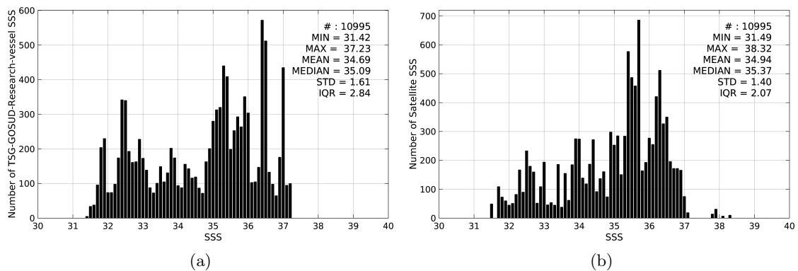
Figure 2: Histograms of SSS from TSG-GOSUD-Research-vessel (a) and SMOS-L3-CATDS-CPDC-V3-10DAYS-25KM (b) considering all match-up pairs per bins of 0.1 over the Gulf Stream Pi-MEP region and for the full satellite product period.
