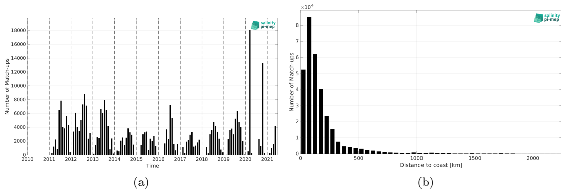
Figure 2: Number of match-ups between TSG (SAMOS) and SMOS SSS L3 v2 - 9-Days (BEC) SSS as a function of time (a) and as function of the distance to coast (b) over the Gulf Stream Pi-MEP region and for the full satellite product period.
