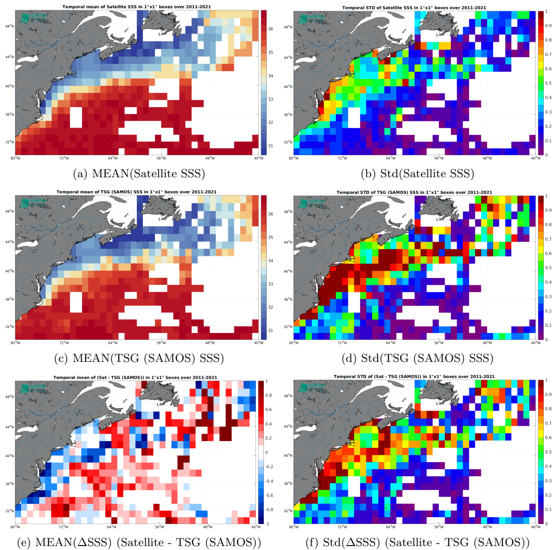
Figure 7: Temporal mean (left) and Std (right) of SSS from SMOS SSS L3 v2 - 9-Days (BEC) (top), TSG (SAMOS) (middle), and of \Delta SSS (Satellite - TSG (SAMOS)). Only match-up pairs are used to generate these maps.
