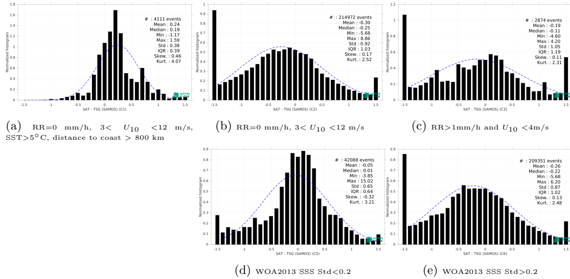
Figure 15: Normalized histogram of \Delta SSS (SMOS SSS L3 v2 - 9-Days (BEC) - TSG (SAMOS)) for 5 different subdatasets corresponding to: RR=0 mm/h, 3 < U_{10} < 12 m/s, SST>5°C, distance to coast > 800 km (a), RR=0 mm/h, 3 < U_{10} < 12 m/s (b), RR>1mm/h and U_{10} < 4 m/s (c), WOA2013 SSS Std<0.2 (d), WOA2013 SSS Std>0.2 (e).
