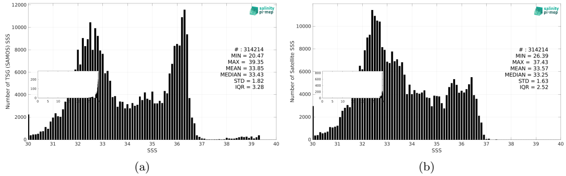
Figure 3: Histograms of SSS from TSG (SAMOS) (a) and SMOS SSS L3 v2 - 9-Days (BEC) (b) considering all match-up pairs per bins of 0.1 over the Gulf Stream Pi-MEP region and for the full satellite product period.
