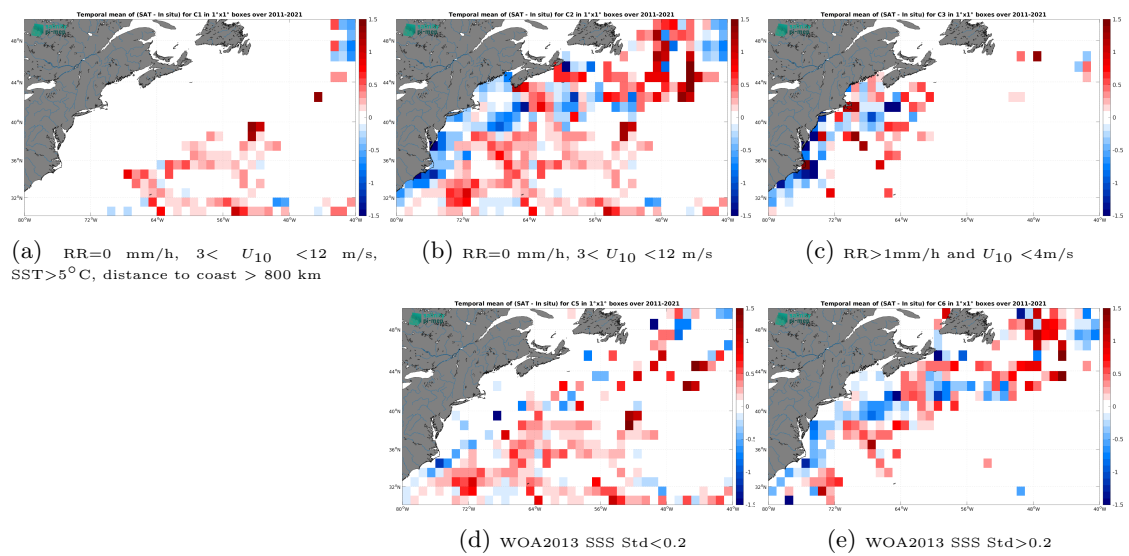
Figure 14: Temporal mean gridded over spatial boxes of size 1^\circ \times 1^\circ of \Delta SSS (SMOS SSS L3 v2 - 9-Days (BEC) - TSG (SAMOS)) for 5 different subdatasets corresponding to:RR=0 mm/h, 3 < U_{10} < 12 m/s, SST>5°C, distance to coast > 800 km (a), RR=0 mm/h, 3 < U_{10} < 12 m/s (b), RR>1mm/h and U_{10} < 4 m/s (c), WOA2013 SSS Std<0.2 (d), WOA2013 SSS Std>0.2 (e).
