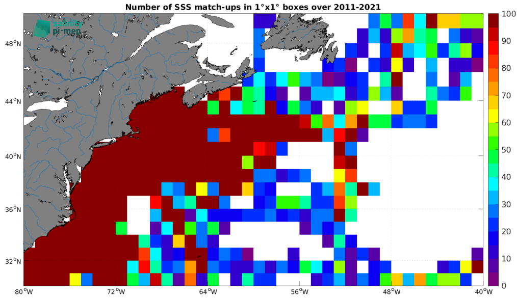
Figure 5: Number of SSS match-ups between TSG (SAMOS) SSS and the SMOS SSS L3 v2 - 9-Days (BEC) SSS product for the Gulf Stream Pi-MEP region over 1^\circ \times 1^\circ boxes and for the full satellite product period.
