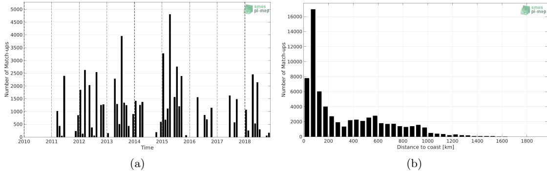
Figure 1: Number of match-ups between TSG (LEGOS-DM) and SMOS SSS L3 v2 - 9-Days (BEC) SSS as a function of time (a) and as function of the distance to coast (b) over the Gulf Stream Pi-MEP region and for the full satellite product period.
