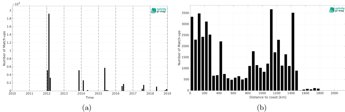
Figure 2: Number of match-ups between TSG (GOSUD-Sailing-ship) and SMOS SSS L3 v2 - 9-Days (BEC) SSS as a function of time (a) and as function of the distance to coast (b) over the Gulf Stream Pi-MEP region and for the full satellite product period.
