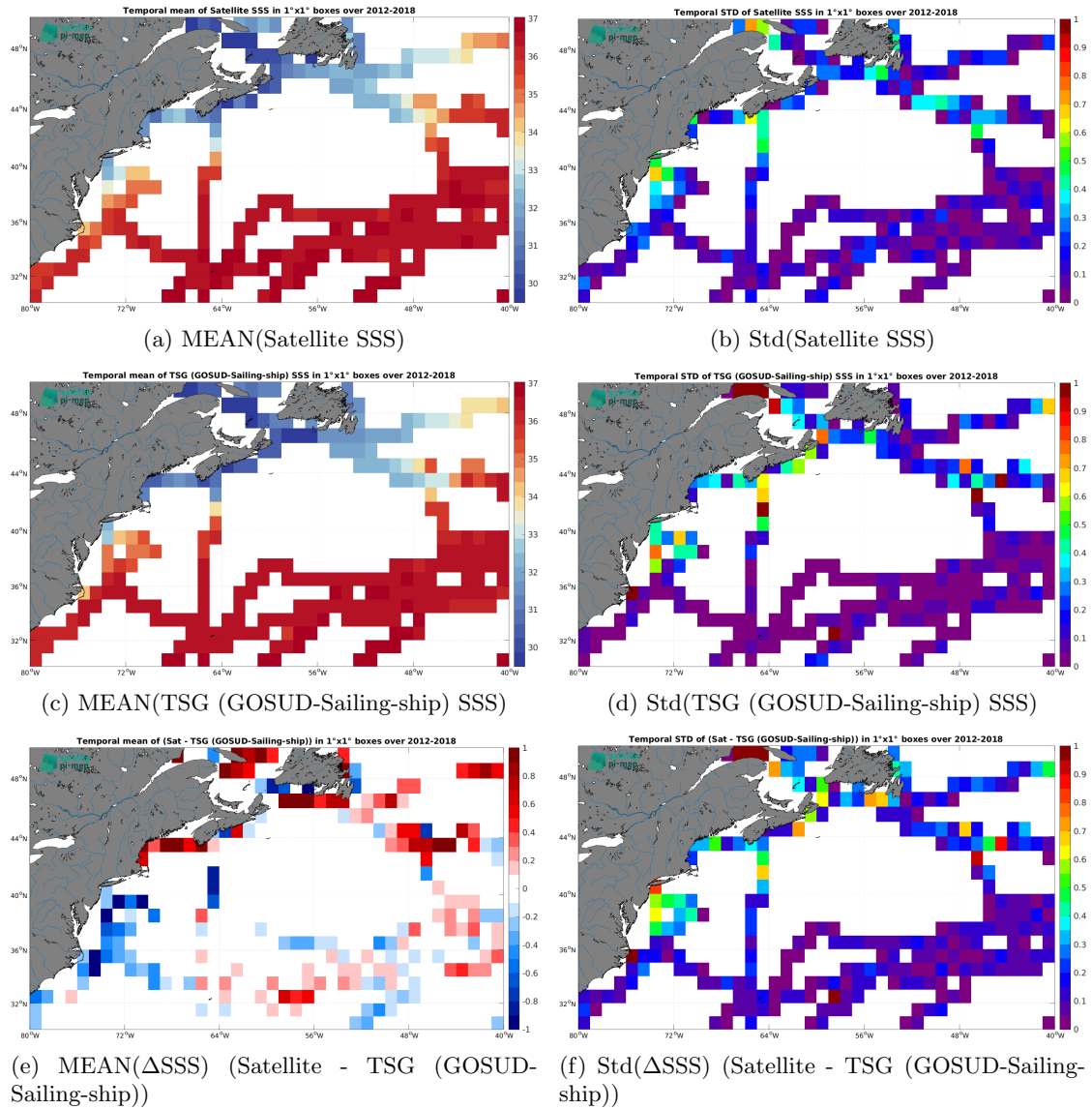
Figure 7: Temporal mean (left) and Std (right) of SSS from SMOS SSS L3 v2 - 9-Days (BEC) (top), TSG (GOSUD-Sailing-ship) (middle), and of \Delta SSS (Satellite - TSG (GOSUD-Sailing-ship)). Only match-up pairs are used to generate these maps.
