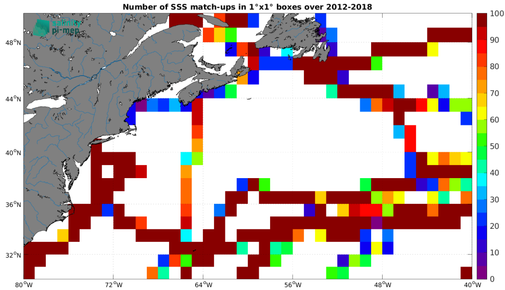
Figure 5: Number of SSS match-ups between TSG (GOSUD-Sailing-ship) SSS and the SMOS SSS L3 v2 - 9-Days (BEC) SSS product for the Gulf Stream Pi-MEP region over 1^\circ \times 1^\circ boxes and for the full satellite product period.
