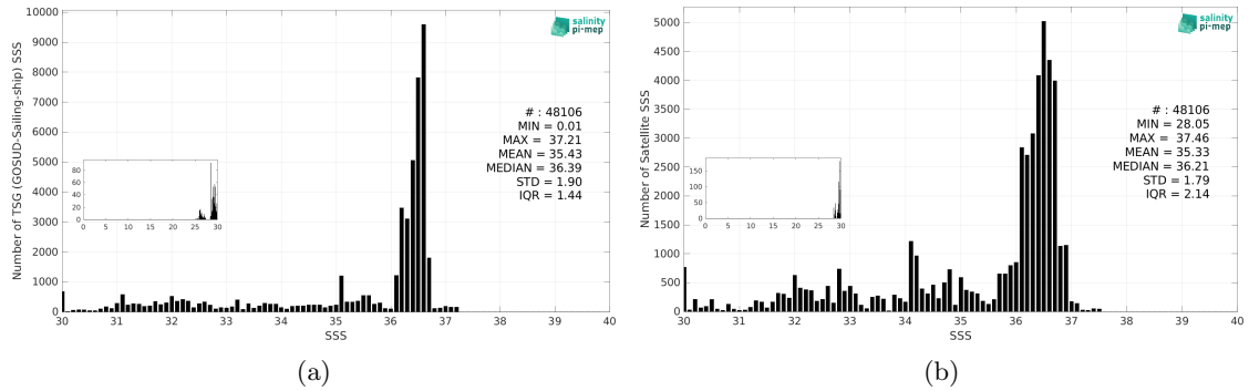
Figure 3: Histograms of SSS from TSG (GOSUD-Sailing-ship) (a) and SMOS SSS L3 v2 - 9-Days (BEC) (b) considering all match-up pairs per bins of 0.1 over the Gulf Stream Pi-MEP region and for the full satellite product period.
