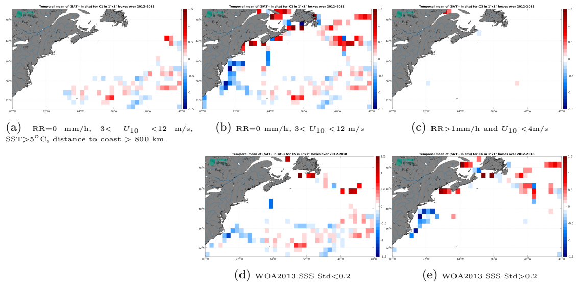
Figure 14: Temporal mean gridded over spatial boxes of size 1^\circ \times 1^\circ of \Delta SSS (SMOS SSS L3 v2 - 9-Days (BEC) - TSG (GOSUD-Sailing-ship)) for 5 different subdatasets corresponding to:RR=0 mm/h, 3 < U_{10} < 12 m/s, SST > 5°C, distance to coast > 800 km (a), RR=0 mm/h, 3 < U_{10} < 12 m/s (b), RR > 1mm/h and U_{10} < 4 m/s (c), WOA2013 SSS Std < 0.2 (d), WOA2013 SSS Std > 0.2 (e).
