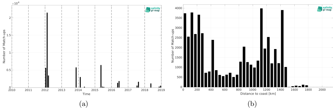
Figure 1: Number of match-ups between TSG (GOSUD-Sailing-ship) and SMOS SSS L3 v2 - 9-Days (BEC) SSS as a function of time (a) and as function of the distance to coast (b) over the Gulf Stream Pi-MEP region and for the full satellite product period.
