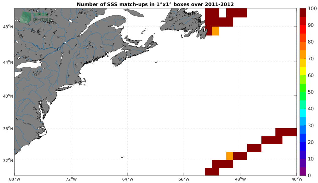
Figure 4: Number of SSS match-ups between TSG (CSIC-UTM) SSS and the SMOS SSS L3 v2 - 9-Days (BEC) SSS product for the Gulf Stream Pi-MEP region over 1^\circ \times 1^\circ boxes and for the full satellite product period.
