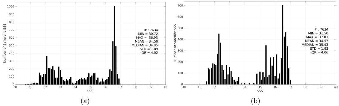
Figure 3: Histograms of SSS from Saildrone (a) and SMOS SSS L3 v2 - 9-Days (BEC) (b) considering all match-up pairs per bins of 0.1 over the Gulf Stream Pi-MEP region and for the full satellite product period.
