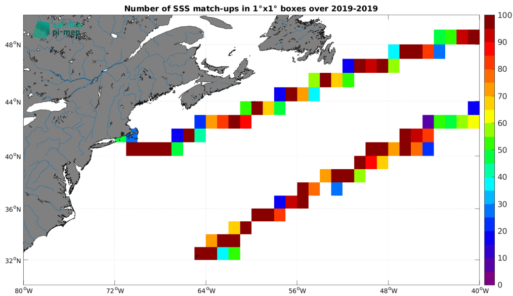
Figure 5: Number of SSS match-ups between Saildrone SSS and the SMOS SSS L3 v2 - 9-Days (BEC) SSS product for the Gulf Stream Pi-MEP region over 1^{\circ} \times 1^{\circ} boxes and for the full satellite product period.
