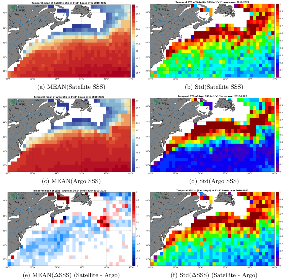
Figure 6: Temporal mean (left) and Std (right) of SSS from SMOS SSS L2-AVERAGED v700 (ESA) (top), Argo (middle), and of \Delta SSS (Satellite - Argo). Only match-up pairs are used to generate these maps.
