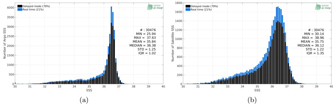
Figure 2: Histograms of SSS from Argo (a) and SMOS SSS L2-AVERAGED v700 (ESA) (b) considering all match-up pairs per bins of 0.1 over the Gulf Stream Pi-MEP region and for the full satellite product period.
