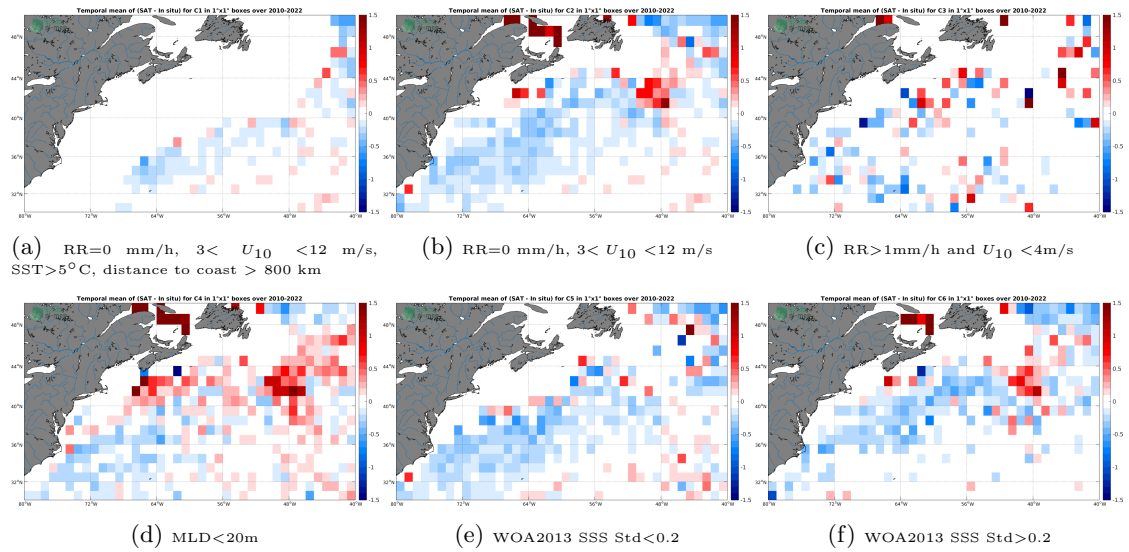
Figure 12: Temporal mean gridded over spatial boxes of size 1^\circ \times 1^\circ of \Delta SSS (SMOS SSS L2-AVERAGED v700 (ESA) - Argo) for 6 different subdatasets corresponding to:RR=0 mm/h, 3 < U_{10} < 12 m/s, SST > 5^\circ\text{C} , distance to coast > 800 km (a), RR=0 mm/h, 3 < U_{10} < 12 m/s (b), RR > 1 mm/h and U_{10} < 4 m/s (c),MLD < 20 m (d),WOA2013 SSS Std < 0.2 (e),WOA2013 SSS Std > 0.2 (f).
