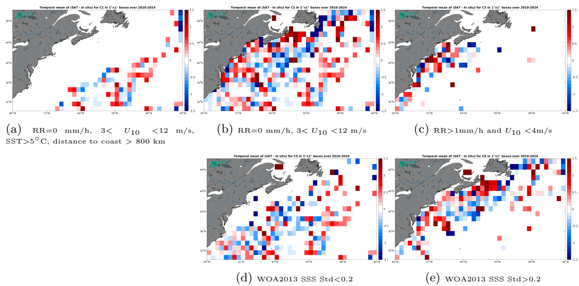
Figure 14: Temporal mean gridded over spatial boxes of size 1^\circ \times 1^\circ of \Delta SSS (SMOS SSS L2 v700 (ESA) - TSG (SAMOS)) for 5 different subdatasets corresponding to:RR=0 mm/h, 3 < U_{10} < 12 m/s, SST>5°C, distance to coast > 800 km (a), RR=0 mm/h, 3 < U_{10} < 12 m/s (b), RR>1mm/h and U_{10} < 4 m/s (c), WOA2013 SSS Std<0.2 (d), WOA2013 SSS Std>0.2 (e).
