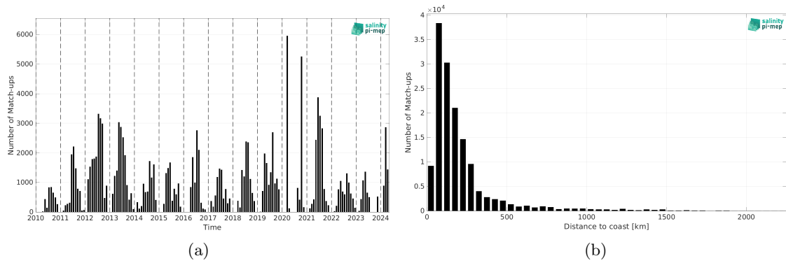
Figure 2: Number of match-ups between TSG (SAMOS) and SMOS SSS L2 v700 (ESA) SSS as a function of time (a) and as function of the distance to coast (b) over the Gulf Stream Pi-MEP region and for the full satellite product period.
