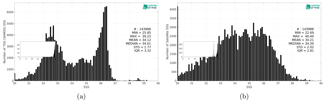
Figure 3: Histograms of SSS from TSG (SAMOS) (a) and SMOS SSS L2 v700 (ESA) (b) considering all match-up pairs per bins of 0.1 over the Gulf Stream Pi-MEP region and for the full satellite product period.
