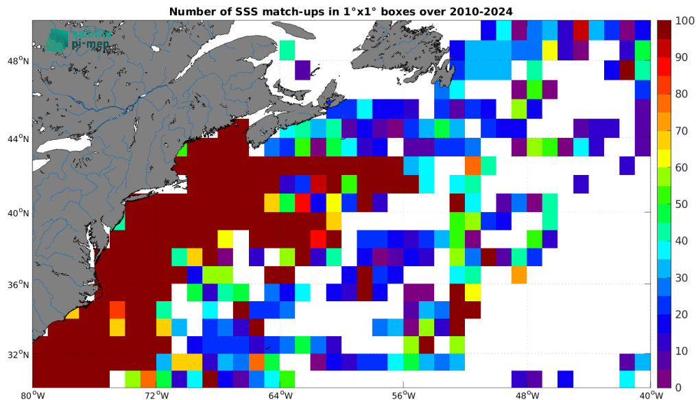
Figure 5: Number of SSS match-ups between TSG (SAMOS) SSS and the SMOS SSS L2 v700 (ESA) SSS product for the Gulf Stream Pi-MEP region over 1^\circ \times 1^\circ boxes and for the full satellite product period.
