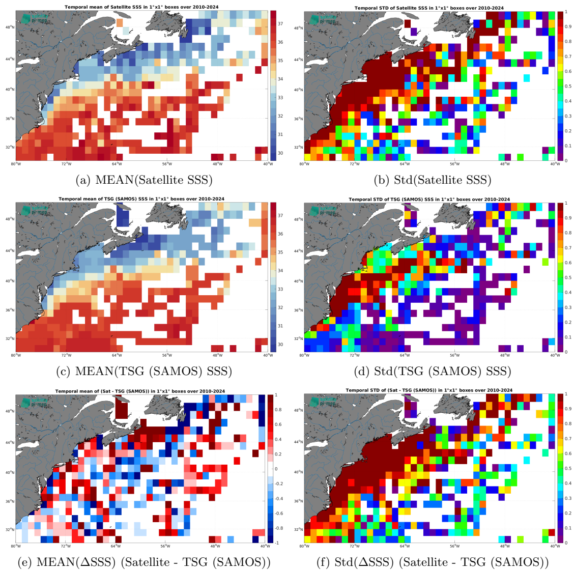
Figure 7: Temporal mean (left) and Std (right) of SSS from SMOS SSS L2 v700 (ESA) (top), TSG (SAMOS) (middle), and of \Delta SSS (Satellite - TSG (SAMOS)). Only match-up pairs are used to generate these maps.
