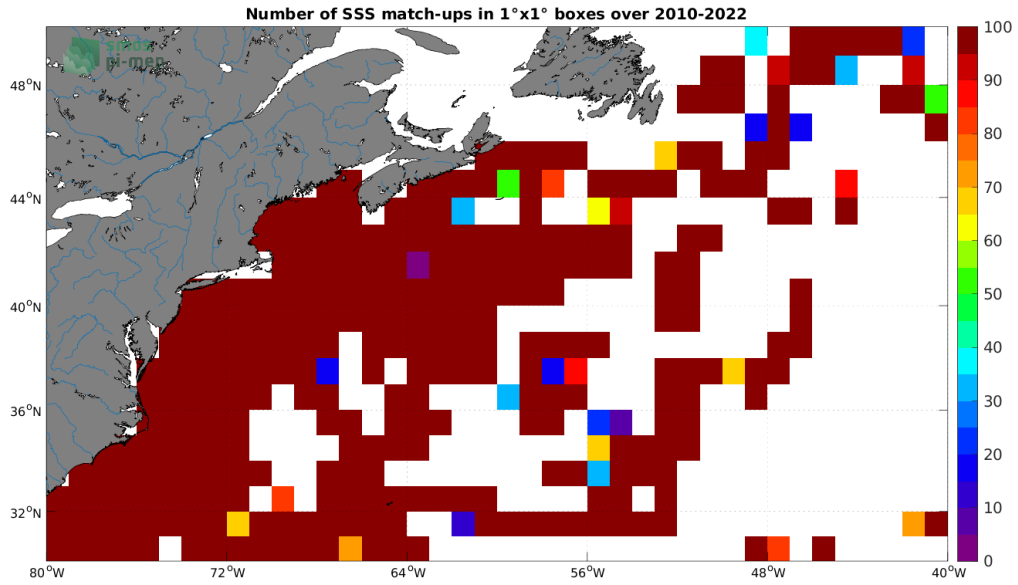
Figure 4: Number of SSS match-ups between TSG (SAMOS) SSS and the SMOS SSS L2 v700 (ESA) SSS product for the Gulf Stream Pi-MEP region over 1^\circ \times 1^\circ boxes and for the full satellite product period.
