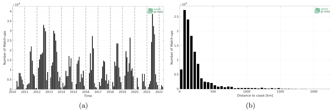
Figure 1: Number of match-ups between TSG (SAMOS) and SMOS SSS L2 v700 (ESA) SSS as a function of time (a) and as function of the distance to coast (b) over the Gulf Stream Pi-MEP region and for the full satellite product period.
