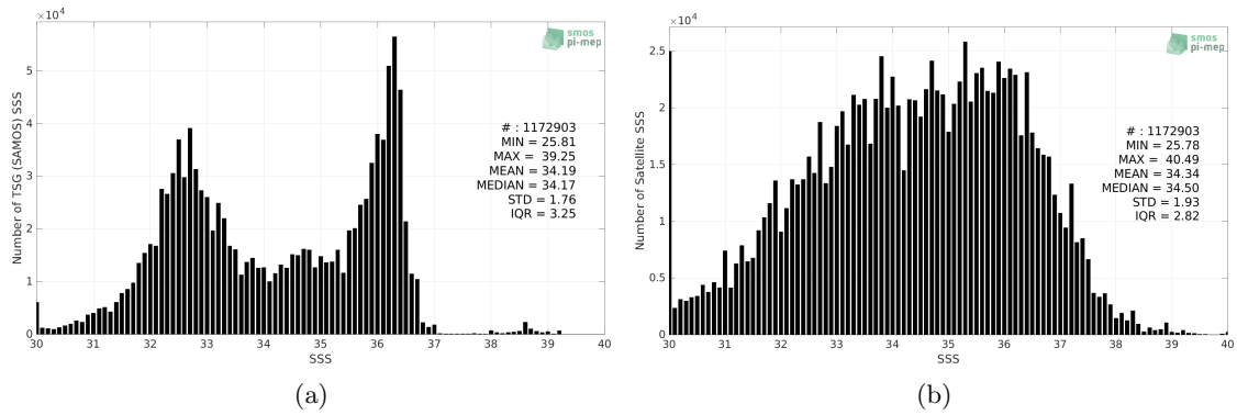
Figure 2: Histograms of SSS from TSG (SAMOS) (a) and SMOS SSS L2 v700 (ESA) (b) considering all match-up pairs per bins of 0.1 over the Gulf Stream Pi-MEP region and for the full satellite product period.
