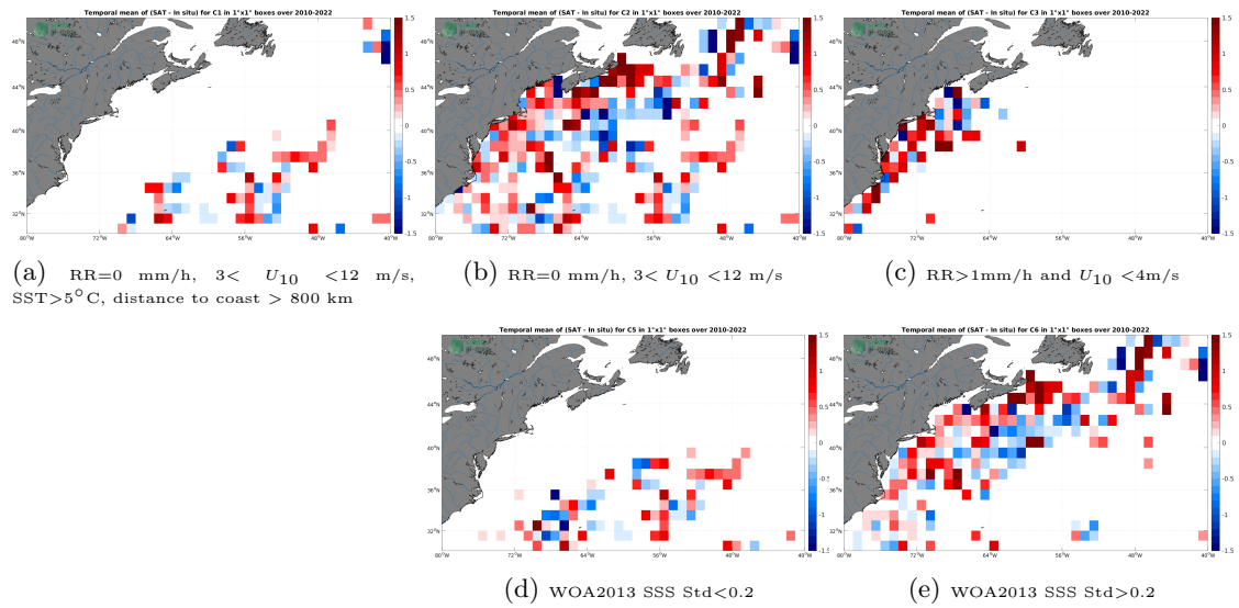
Figure 12: Temporal mean gridded over spatial boxes of size 1^\circ \times 1^\circ of \Delta SSS (SMOS SSS L2 v700 (ESA) - TSG (SAMOS)) for 5 different subdatasets corresponding to:RR=0 mm/h, 3 < U_{10} < 12 m/s, SST >5^\circ C, distance to coast > 800 km (a), RR=0 mm/h, 3 < U_{10} < 12 m/s (b), RR >1 mm/h and U_{10} < 4 m/s (c), WOA2013 SSS Std <0.2 (d), WOA2013 SSS Std >0.2 (e).
