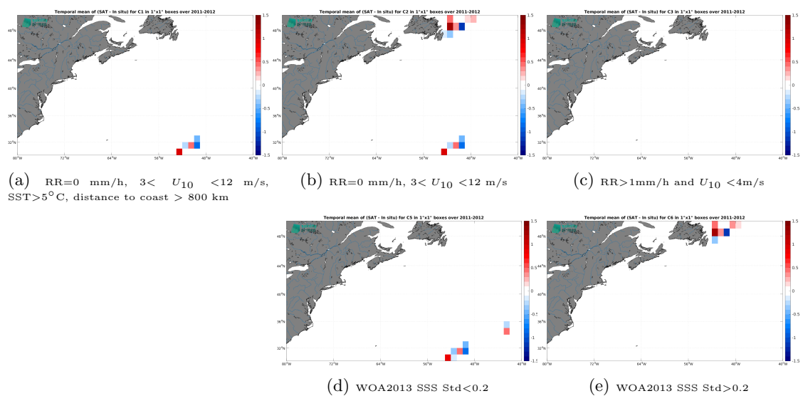
Figure 14: Temporal mean gridded over spatial boxes of size 1^\circ \times 1^\circ of \Delta SSS (SMOS SSS L2 v700 (ESA) - TSG (CSIC-UTM)) for 5 different subdatasets corresponding to: RR=0 mm/h, 3 < U_{10} < 12 m/s, SST > 5°C, distance to coast > 800 km (a), RR=0 mm/h, 3 < U_{10} < 12 m/s (b), RR > 1mm/h and U_{10} < 4 m/s (c), WOA2013 SSS Std < 0.2 (d), WOA2013 SSS Std > 0.2 (e).
