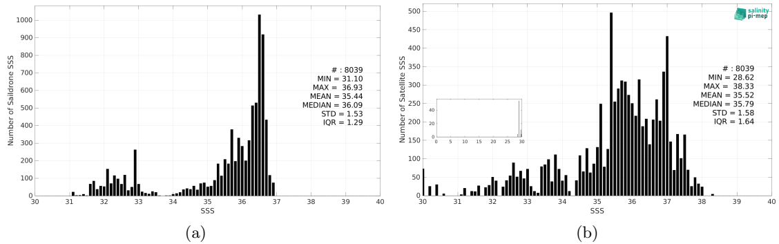
Figure 3: Histograms of SSS from Saildrone (a) and SMOS SSS L2 v700 (ESA) (b) considering all match-up pairs per bins of 0.1 over the Gulf Stream Pi-MEP region and for the full satellite product period.
