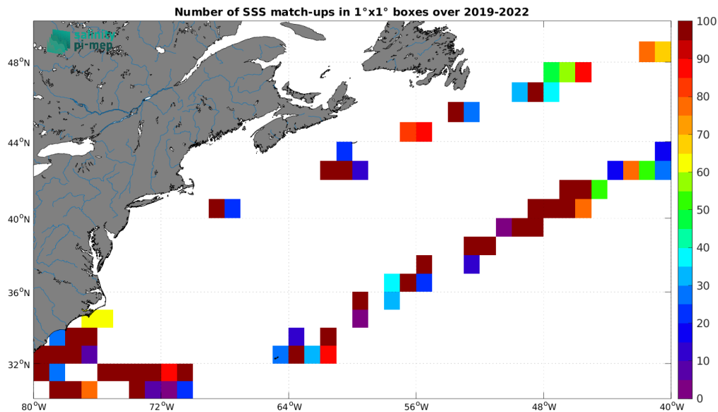
Figure 5: Number of SSS match-ups between Salldrone SSS and the SMOS SSS L2 v700 (ESA) SSS product for the Gulf Stream Pi-MEP region over 1^\circ \times 1^\circ boxes and for the full satellite product period.
