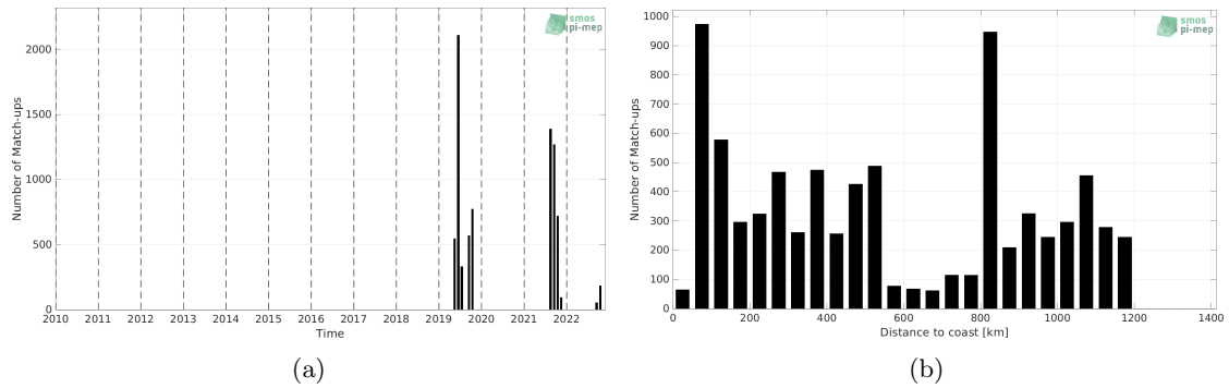
Figure 1: Number of match-ups between Sairdrone and SMOS SSS L2 v700 (ESA) SSS as a function of time (a) and as function of the distance to coast (b) over the Gulf Stream Pi-MEP region and for the full satellite product period.
