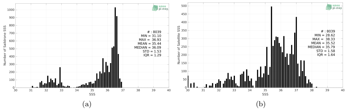
Figure 2: Histograms of SSS from Sairdrone (a) and SMOS SSS L2 v700 (ESA) (b) considering all match-up pairs per bins of 0.1 over the Gulf Stream Pi-MEP region and for the full satellite product period.
