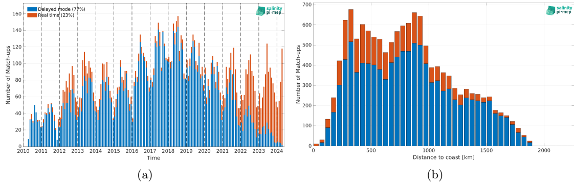
Figure 2: Number of match-ups between Argo and SMOS SSS L2 v700 (ESA) SSS as a function of time (a) and as function of the distance to coast (b) over the Gulf Stream Pi-MEP region and for the full satellite product period.
