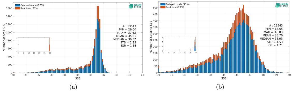
Figure 3: Histograms of SSS from Argo (a) and SMOS SSS L2 v700 (ESA) (b) considering all match-up pairs per bins of 0.1 over the Gulf Stream Pi-MEP region and for the full satellite product period.
