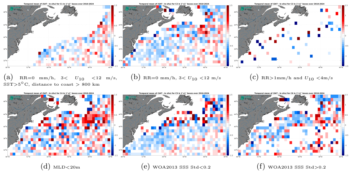
Figure 14: Temporal mean gridded over spatial boxes of size 1^\circ \times 1^\circ of \Delta SSS (SMOS SSS L2 v700 (ESA) - Argo) for 6 different subdatasets corresponding to:RR=0 mm/h, 3 < U_{10} < 12 m/s, SST>5°C, distance to coast > 800 km (a), RR=0 mm/h, 3 < U_{10} < 12 m/s (b), RR>1mm/h and U_{10} < 4 m/s (c),MLD<20m (d),WOA2013 SSS Std<0.2 (e),WOA2013 SSS Std>0.2 (f).
