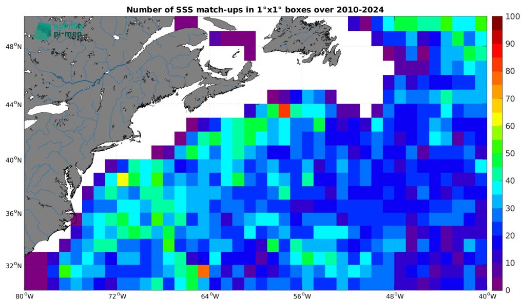
Figure 5: Number of SSS match-ups between Argo SSS and the SMOS SSS L2 v700 (ESA) SSS product for the Gulf Stream Pi-MEP region over 1^\circ \times 1^\circ boxes and for the full satellite product period.
