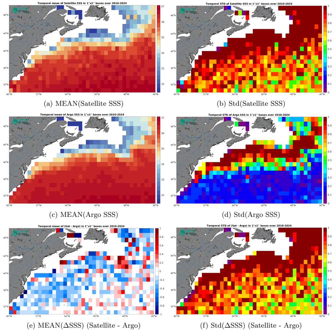
Figure 7: Temporal mean (left) and Std (right) of SSS from SMOS SSS L2 v700 (ESA) (top), Argo (middle), and of \Delta SSS (Satellite - Argo). Only match-up pairs are used to generate these maps.
