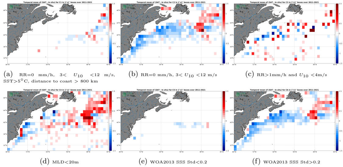
Figure 12: Temporal mean gridded over spatial boxes of size 1^\circ \times 1^\circ of \Delta SSS (SMAP SSS L4 OI v1 - 7 Days (IPRC) - Argo) for 6 different subdatasets corresponding to: RR=0 mm/h, 3 < U_{10} < 12 m/s, SST > 5^\circ C , distance to coast > 800 km (a), RR=0 mm/h, 3 < U_{10} < 12 m/s (b), RR > 1 mm/h and U_{10} < 4 m/s (c), MLD < 20 m (d), WOA2013 SSS Std < 0.2 (e), WOA2013 SSS Std > 0.2 (f).
