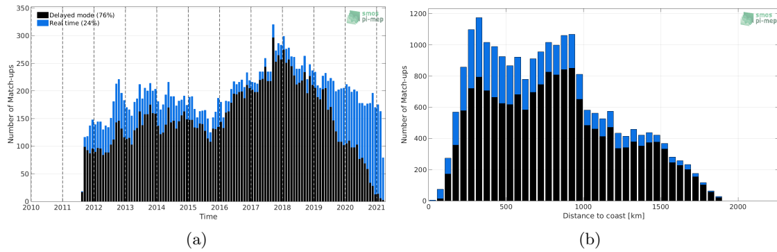
Figure 1: Number of match-ups between Argo and SMAP SSS L4 OI v1 - 7 Days (IPRC) SSS as a function of time (a) and as function of the distance to coast (b) over the Gulf Stream Pi-MEP region and for the full satellite product period.
