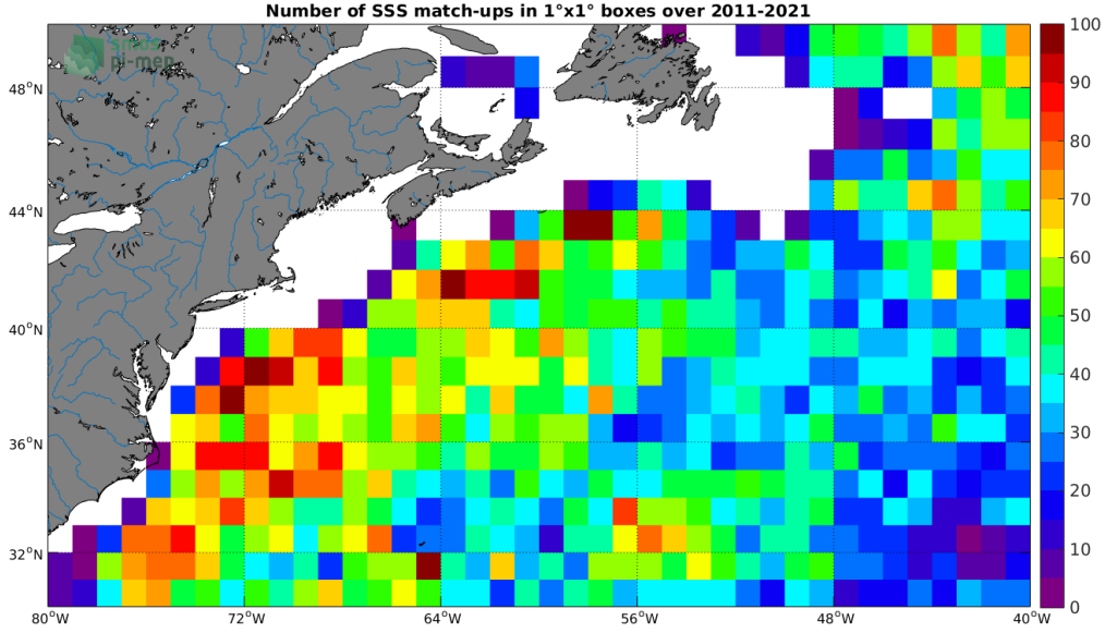
Figure 4: Number of SSS match-ups between Argo SSS and the SMAP SSS L4 OI v1 - 7 Days (IPRC) SSS product for the Gulf Stream Pi-MEP region over 1^\circ \times 1^\circ boxes and for the full satellite product period.
