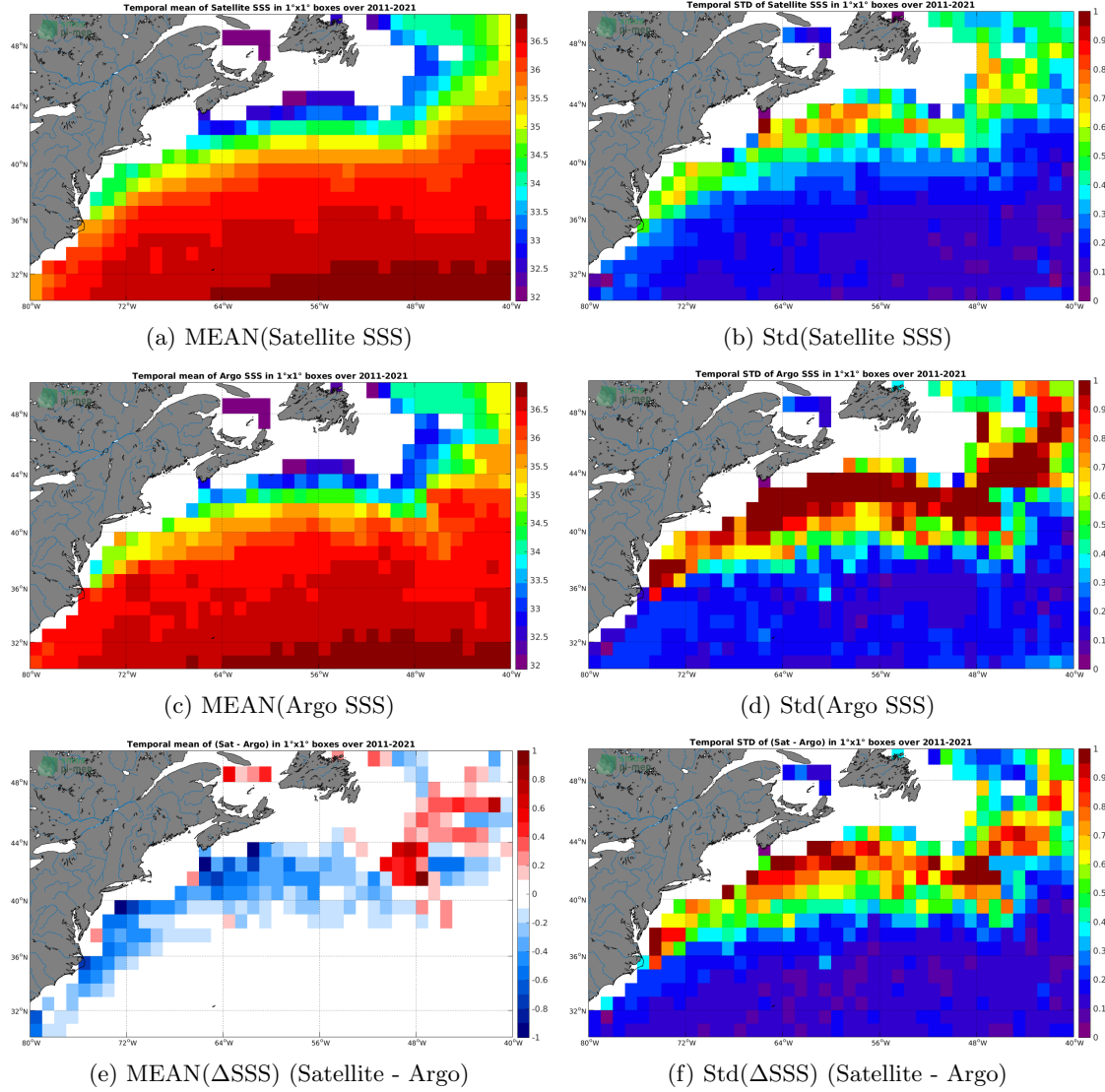
Figure 6: Temporal mean (left) and Std (right) of SSS from SMAP SSS L4 OI v1 - 7 Days (IPRC) (top), Argo (middle), and of \Delta SSS (Satellite - Argo). Only match-up pairs are used to generate these maps.
