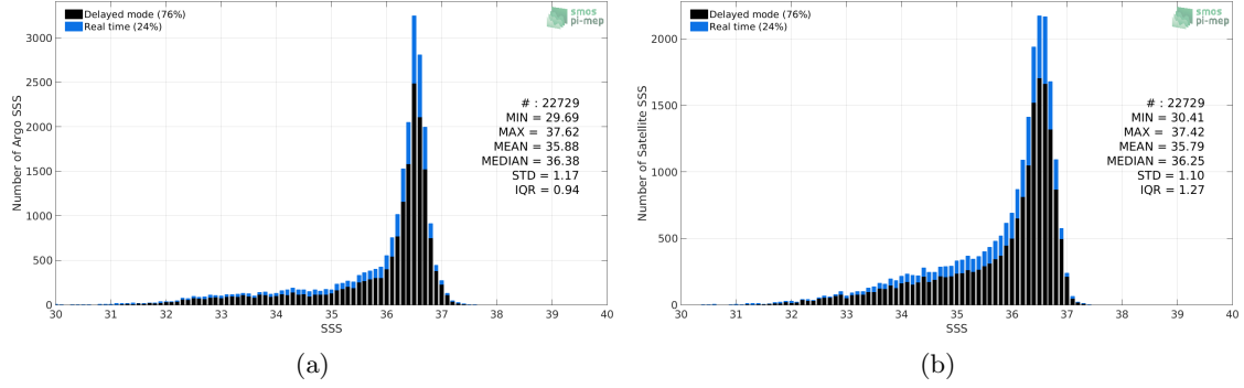
Figure 2: Histograms of SSS from Argo (a) and SMAP SSS L4 OI v1 - 7 Days (IPRC) (b) considering all match-up pairs per bins of 0.1 over the Gulf Stream Pi-MEP region and for the full satellite product period.
