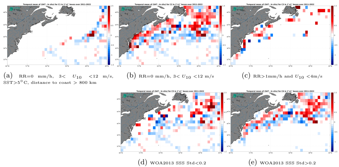
Figure 14: Temporal mean gridded over spatial boxes of size 1^\circ \times 1^\circ of \Delta SSS (SMAP SSS L4 OI v3 - Monthly (ESR) - TSG (LEGOS-DM)) for 5 different subdatasets corresponding to:RR=0 mm/h, 3 < U_{10} < 12 m/s, SST>5°C, distance to coast > 800 km (a), RR=0 mm/h, 3 < U_{10} < 12 m/s (b), RR>1mm/h and U_{10} < 4 m/s (c), WOA2013 SSS Std<0.2 (d), WOA2013 SSS Std>0.2 (e).
