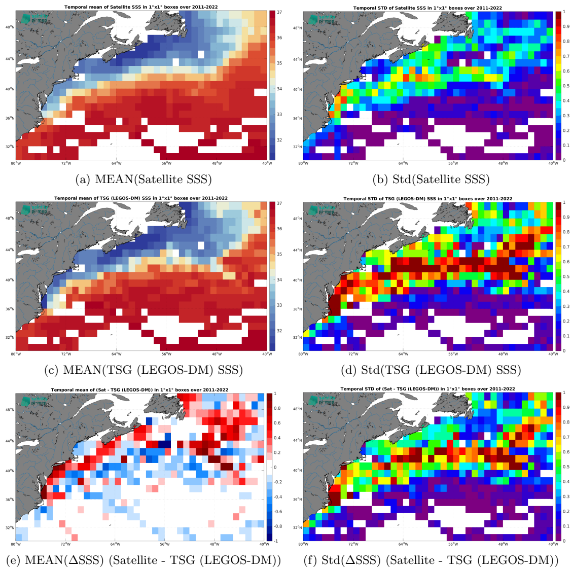
Figure 7: Temporal mean (left) and Std (right) of SSS from SMAP SSS L4 OI v3 - Monthly (ESR) (top), TSG (LEGOS-DM) (middle), and of \Delta SSS (Satellite - TSG (LEGOS-DM)). Only match-up pairs are used to generate these maps.
