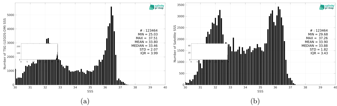
Figure 3: Histograms of SSS from TSG (LEGOS-DM) (a) and SMAP SSS L4 OI v3 - Monthly (ESR) (b) considering all match-up pairs per bins of 0.1 over the Gulf Stream Pi-MEP region and for the full satellite product period.
