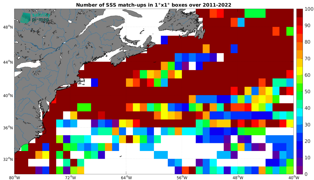
Figure 5: Number of SSS match-ups between TSG (LEGOS-DM) SSS and the SMAP SSS L4 OI v3 - Monthly (ESR) SSS product for the Gulf Stream Pi-MEP region over 1^\circ \times 1^\circ boxes and for the full satellite product period.
