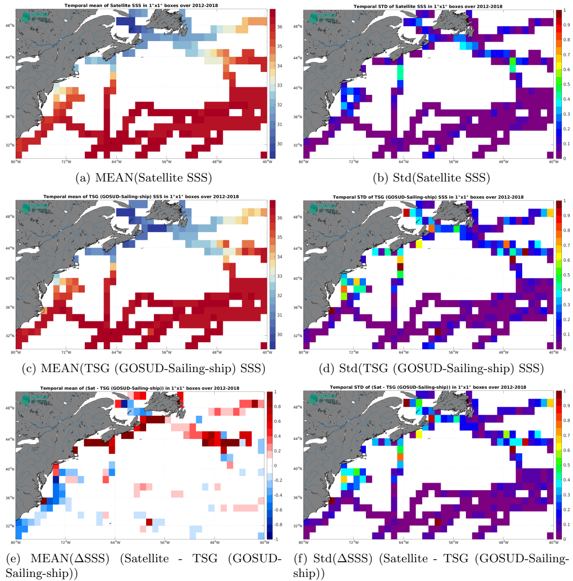
Figure 7: Temporal mean (left) and Std (right) of SSS from SMAP SSS L4 OI v3 - Monthly (ESR) (top), TSG (GOSUD-Sailing-ship) (middle), and of \Delta SSS (Satellite - TSG (GOSUD-Sailing-ship)). Only match-up pairs are used to generate these maps.
