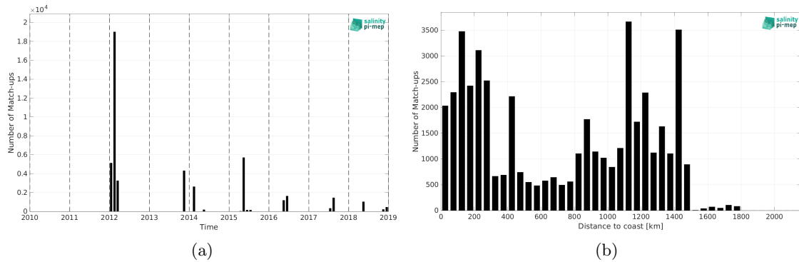
Figure 2: Number of match-ups between TSG (GOSUD-Sailing-ship) and SMAP SSS L4 OI v3 - Monthly (ESR) SSS as a function of time (a) and as function of the distance to coast (b) over the Gulf Stream Pi-MEP region and for the full satellite product period.
