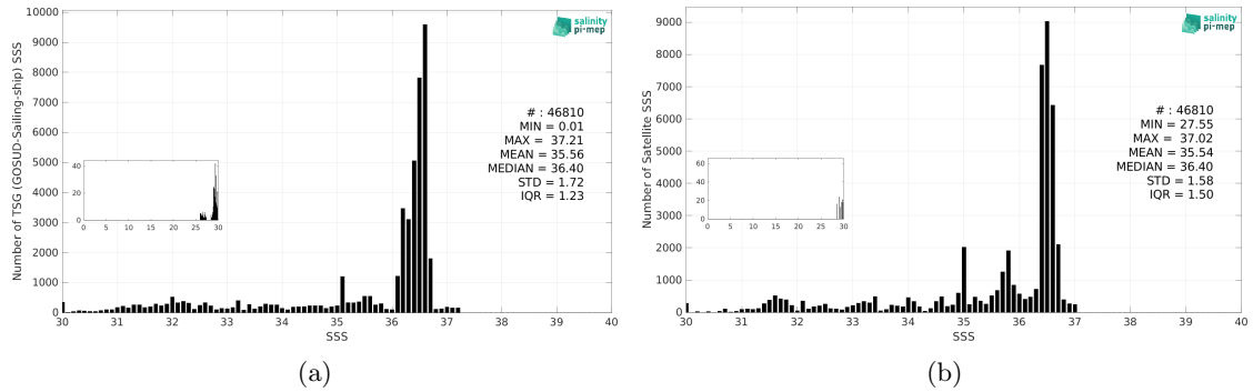
Figure 3: Histograms of SSS from TSG (GOSUD-Sailing-ship) (a) and SMAP SSS L4 OI v3 - Monthly (ESR) (b) considering all match-up pairs per bins of 0.1 over the Gulf Stream Pi-MEP region and for the full satellite product period.
