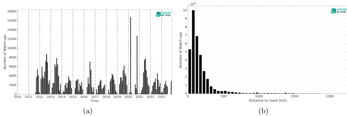
Figure 2: Number of match-ups between TSG (SAMOS) and SMAP SSS L4 OI v3 - Daily (ESR) SSS as a function of time (a) and as function of the distance to coast (b) over the Gulf Stream Pi-MEP region and for the full satellite product period.
