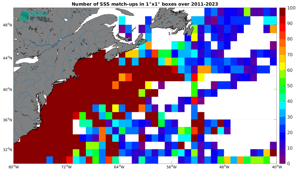
Figure 5: Number of SSS match-ups between TSG (SAMOS) SSS and the SMAP SSS L4 OI v3 - Daily (ESR) SSS product for the Gulf Stream Pi-MEP region over 1^\circ \times 1^\circ boxes and for the full satellite product period.
