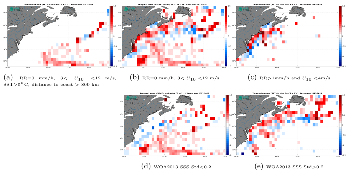
Figure 14: Temporal mean gridded over spatial boxes of size 1^\circ \times 1^\circ of \Delta SSS (SMAP SSS L4 OI v3 - Daily (ESR) - TSG (SAMOS)) for 5 different subdatasets corresponding to: RR=0 mm/h, 3 < U_{10} < 12 m/s, SST > 5°C, distance to coast > 800 km (a), RR=0 mm/h, 3 < U_{10} < 12 m/s (b), RR > 1mm/h and U_{10} < 4 m/s (c), WOA2013 SSS Std < 0.2 (d), WOA2013 SSS Std > 0.2 (e).
