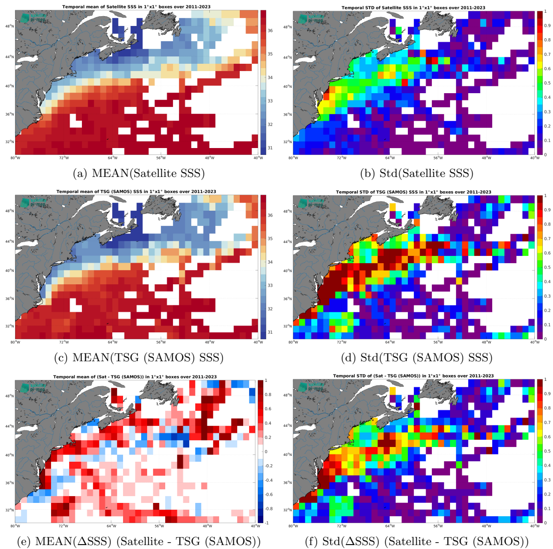
Figure 7: Temporal mean (left) and Std (right) of SSS from SMAP SSS L4 OI v3 - Daily (ESR) (top), TSG (SAMOS) (middle), and of \Delta SSS (Satellite - TSG (SAMOS)). Only match-up pairs are used to generate these maps.
