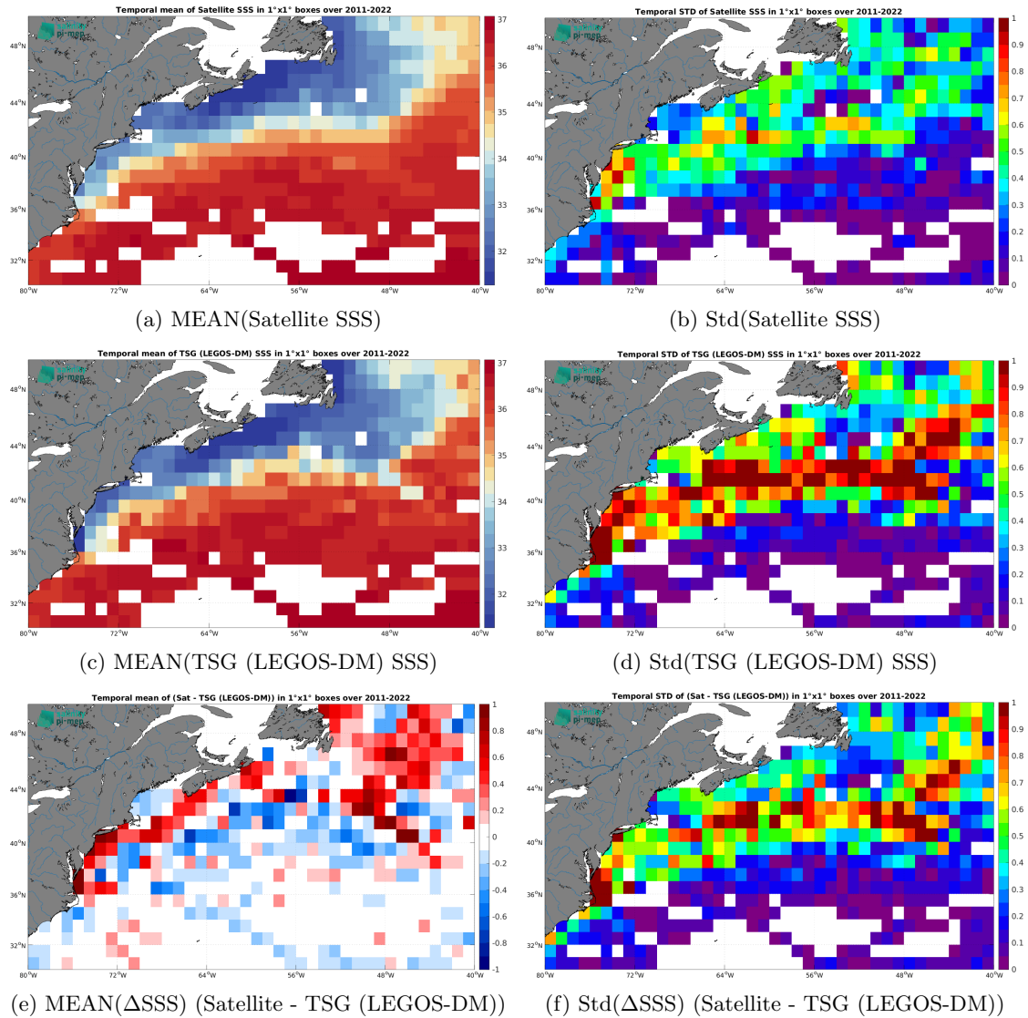
Figure 7: Temporal mean (left) and Std (right) of SSS from SMAP SSS L4 OI v3 - Daily (ESR) (top), TSG (LEGOS-DM) (middle), and of \Delta SSS (Satellite - TSG (LEGOS-DM)). Only match-up pairs are used to generate these maps.
