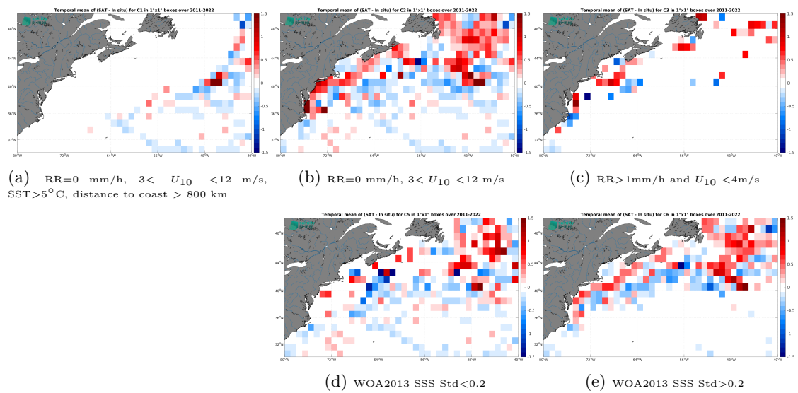
Figure 14: Temporal mean gridded over spatial boxes of size 1^\circ \times 1^\circ of \Delta SSS (SMAP SSS L4 OI v3 - Daily (ESR) - TSG (LEGOS-DM)) for 5 different subdatasets corresponding to:RR=0 mm/h, 3 < U_{10} < 12 m/s, SST > 5°C, distance to coast > 800 km (a), RR=0 mm/h, 3 < U_{10} < 12 m/s (b), RR > 1mm/h and U_{10} < 4 m/s (c), WOA2013 SSS Std < 0.2 (d), WOA2013 SSS Std > 0.2 (e).
