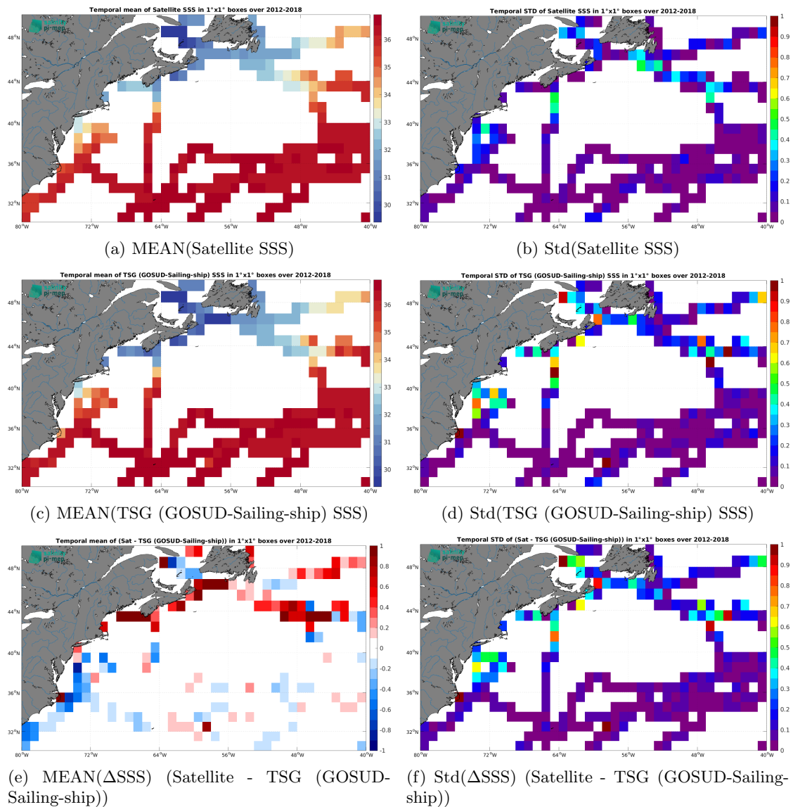
Figure 7: Temporal mean (left) and Std (right) of SSS from SMAP SSS L4 OI v3 - Daily (ESR) (top), TSG (GOSUD-Sailing-ship) (middle), and of \Delta SSS (Satellite - TSG (GOSUD-Sailing-ship)). Only match-up pairs are used to generate these maps.
