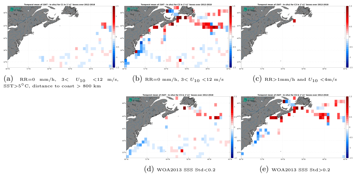
Figure 14: Temporal mean gridded over spatial boxes of size 1^\circ \times 1^\circ of \Delta SSS (SMAP SSS L4 OI v3 - Daily (ESR) - TSG (GOSUD-Sailing-ship)) for 5 different subdatasets corresponding to: RR=0 mm/h, 3 < U_{10} < 12 m/s, SST > 5°C, distance to coast > 800 km (a), RR=0 mm/h, 3 < U_{10} < 12 m/s (b), RR > 1mm/h and U_{10} < 4 m/s (c), WOA2013 SSS Std < 0.2 (d), WOA2013 SSS Std > 0.2 (e).
