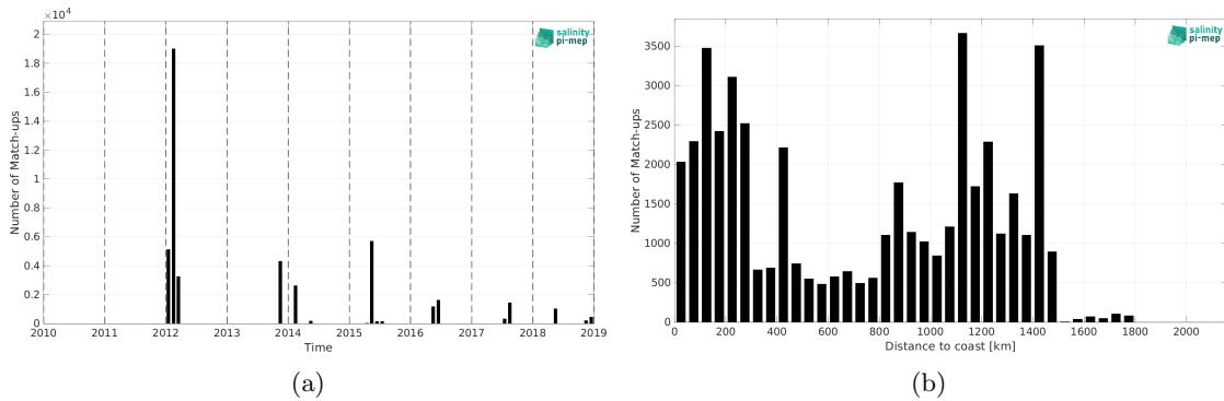
Figure 2: Number of match-ups between TSG (GOSUD-Sailing-ship) and SMAP SSS L4 OI v3 - Daily (ESR) SSS as a function of time (a) and as function of the distance to coast (b) over the Gulf Stream Pi-MEP region and for the full satellite product period.
