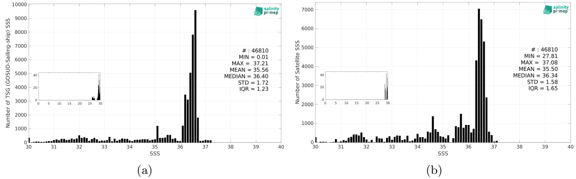
Figure 3: Histograms of SSS from TSG (GOSUD-Sailing-ship) (a) and SMAP SSS L4 OI v3 - Daily (ESR) (b) considering all match-up pairs per bins of 0.1 over the Gulf Stream Pi-MEP region and for the full satellite product period.
