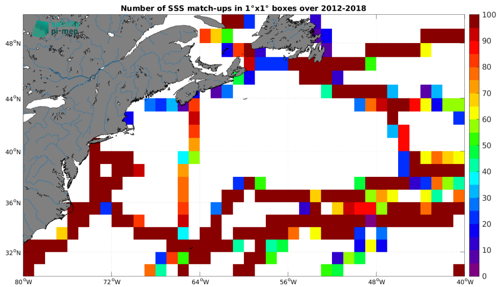
Figure 5: Number of SSS match-ups between TSG (GOSUD-Sailing-ship) SSS and the SMAP SSS L4 OI v3 - Daily (ESR) SSS product for the Gulf Stream Pi-MEP region over 1^\circ \times 1^\circ boxes and for the full satellite product period.
