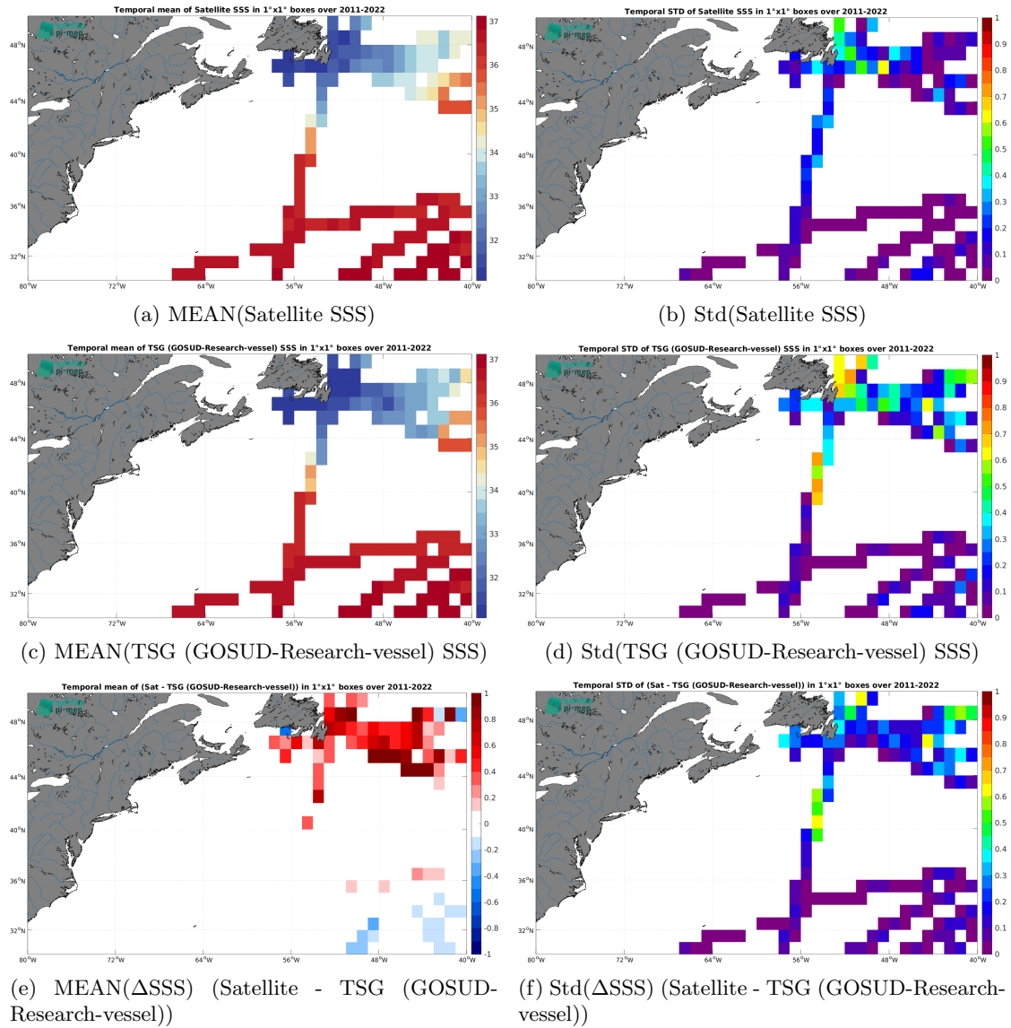
Figure 7: Temporal mean (left) and Std (right) of SSS from SMAP SSS L4 OI v3 - Daily (ESR) (top), TSG (GOSUD-Research-vessel) (middle), and of \Delta SSS (Satellite - TSG (GOSUD-Research-vessel)). Only match-up pairs are used to generate these maps.
