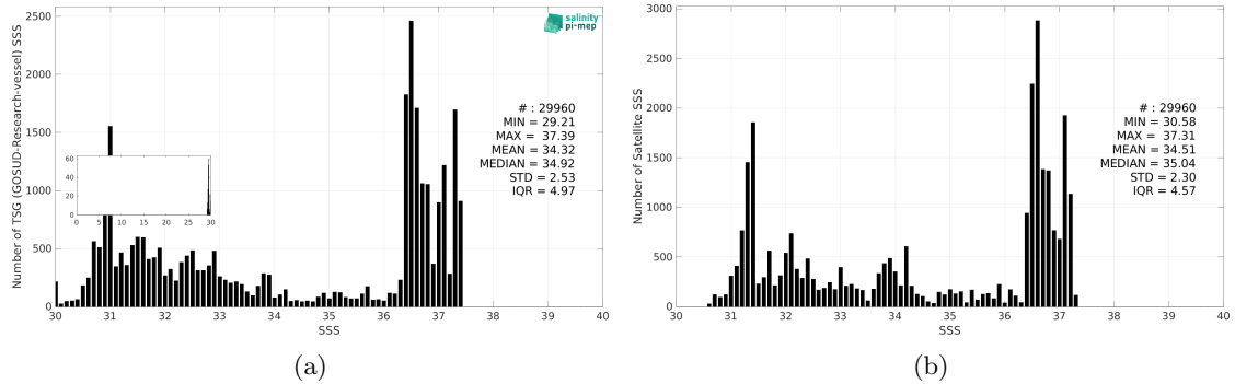
Figure 3: Histograms of SSS from TSG (GOSUD-Research-vessel) (a) and SMAP SSS L4 OI v3 - Daily (ESR) (b) considering all match-up pairs per bins of 0.1 over the Gulf Stream Pi-MEP region and for the full satellite product period.
