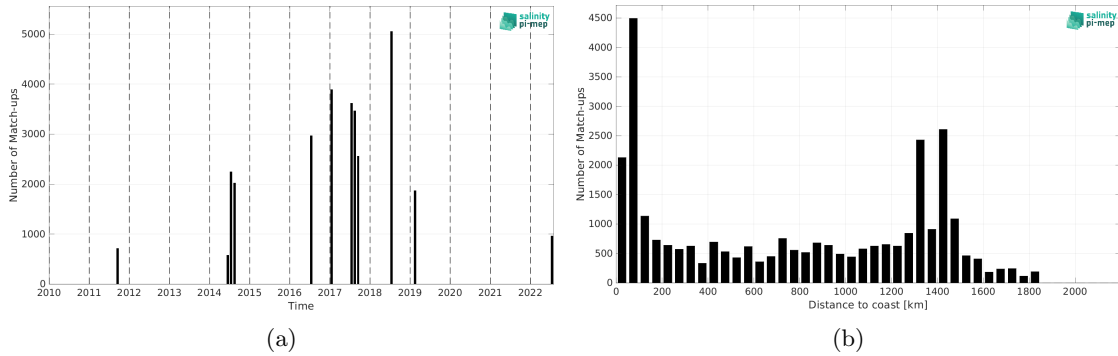
Figure 2: Number of match-ups between TSG (GOSUD-Research-vessel) and SMAP SSS L4 OI v3 - Daily (ESR) SSS as a function of time (a) and as function of the distance to coast (b) over the Gulf Stream Pi-MEP region and for the full satellite product period.
