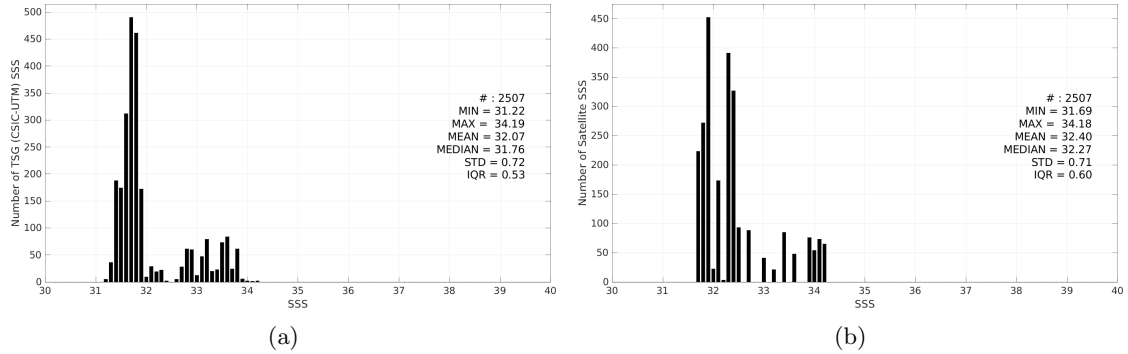
Figure 3: Histograms of SSS from TSG (CSIC-UTM) (a) and SMAP SSS L4 OI v3 - Daily (ESR) (b) considering all match-up pairs per bins of 0.1 over the Gulf Stream Pi-MEP region and for the full satellite product period.
