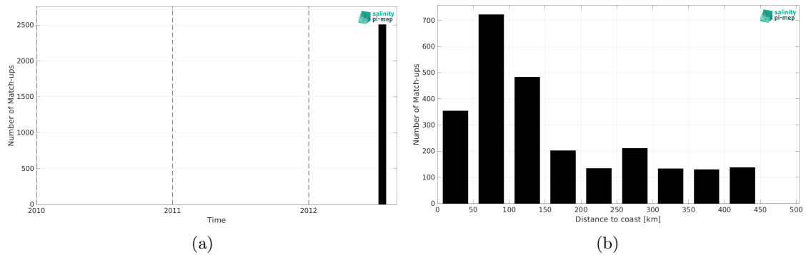
Figure 2: Number of match-ups between TSG (CSIC-UTM) and SMAP SSS L4 OI v3 - Daily (ESR) SSS as a function of time (a) and as function of the distance to coast (b) over the Gulf Stream Pi-MEP region and for the full satellite product period.
