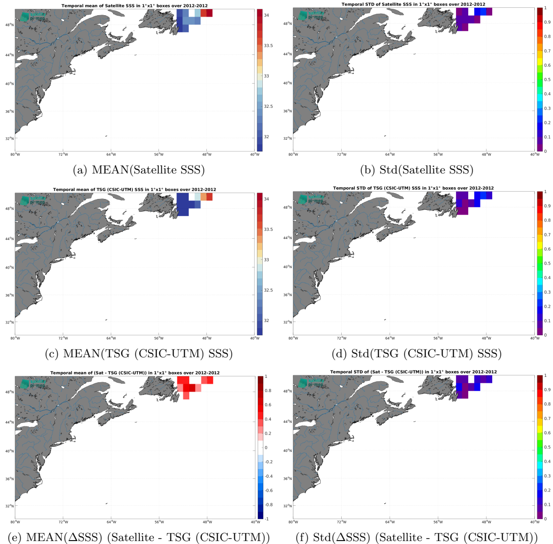
Figure 7: Temporal mean (left) and Std (right) of SSS from SMAP SSS L4 OI v3 - Daily (ESR) (top), TSG (CSIC-UTM) (middle), and of \Delta SSS (Satellite - TSG (CSIC-UTM)). Only match-up pairs are used to generate these maps.
