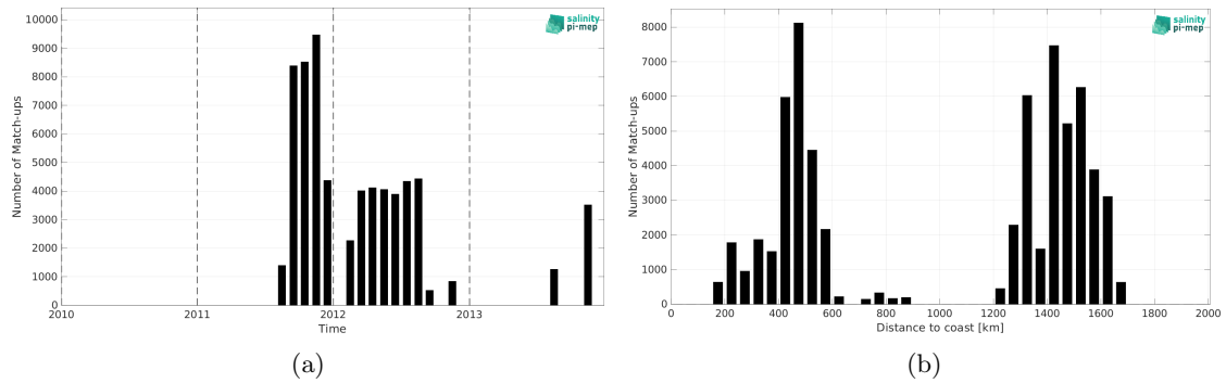
Figure 2: Number of match-ups between Surface drifters and SMAP SSS L4 OI v3 - Daily (ESR) SSS as a function of time (a) and as function of the distance to coast (b) over the Gulf Stream Pi-MEP region and for the full satellite product period.
