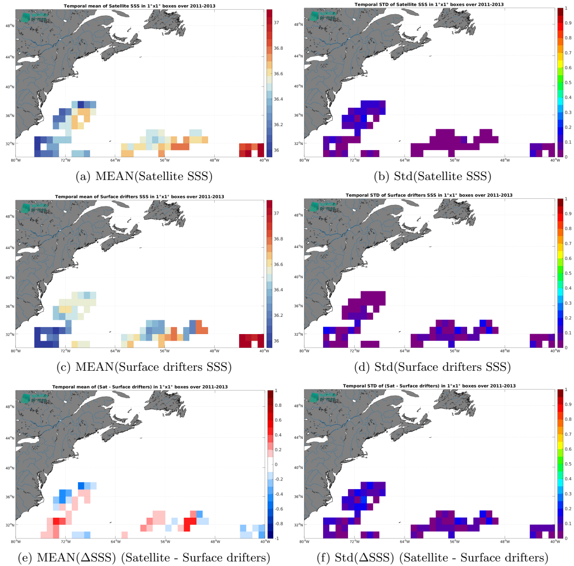
Figure 6: Temporal mean (left) and Std (right) of SSS from SMAP SSS L4 OI v3 - Daily (ESR) (top), Surface drifters (middle), and of \Delta SSS (Satellite - Surface drifters). Only match-up pairs are used to generate these maps.
