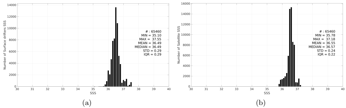
Figure 3: Histograms of SSS from Surface drifters (a) and SMAP SSS L4 OI v3 - Daily (ESR) (b) considering all match-up pairs per bins of 0.1 over the Gulf Stream Pi-MEP region and for the full satellite product period.
