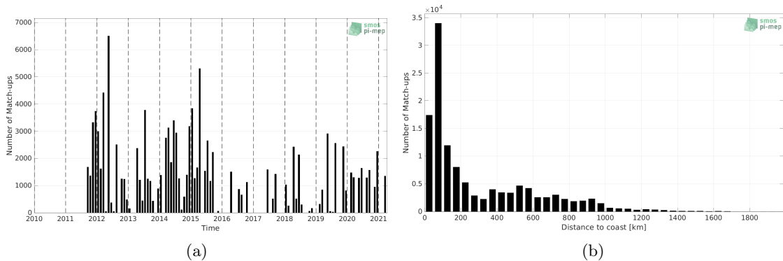
Figure 1: Number of match-ups between TSG (LEGOS-DM) and SMAP SSS L4 OI v2 - 7 Days (ESR) SSS as a function of time (a) and as function of the distance to coast (b) over the Gulf Stream Pi-MEP region and for the full satellite product period.
