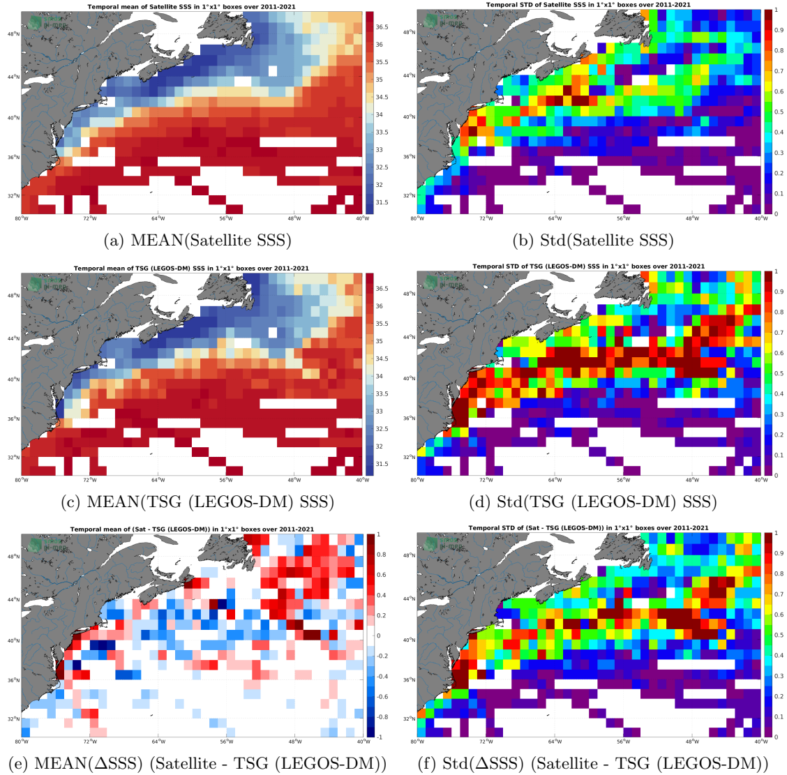
Figure 6: Temporal mean (left) and Std (right) of SSS from SMAP SSS L4 OI v2 - 7 Days (ESR) (top), TSG (LEGOS-DM) (middle), and of \Delta SSS (Satellite - TSG (LEGOS-DM)). Only match-up pairs are used to generate these maps.
