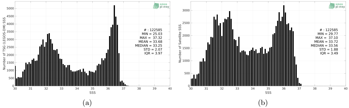
Figure 2: Histograms of SSS from TSG (LEGOS-DM) (a) and SMAP SSS L4 OI v2 - 7 Days (ESR) (b) considering all match-up pairs per bins of 0.1 over the Gulf Stream Pi-MEP region and for the full satellite product period.
