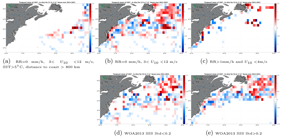
Figure 12: Temporal mean gridded over spatial boxes of size 1^\circ \times 1^\circ of \Delta SSS (SMAP SSS L4 OI v2 - 7 Days (ESR) - TSG (LEGOS-DM)) for 5 different subdatasets corresponding to:RR=0 mm/h, 3 < U_{10} < 12 m/s, SST >5^\circ C, distance to coast > 800 km (a), RR=0 mm/h, 3 < U_{10} < 12 m/s (b), RR >1 mm/h and U_{10} < 4 m/s (c), WOA2013 SSS Std <0.2 (d), WOA2013 SSS Std >0.2 (e).
