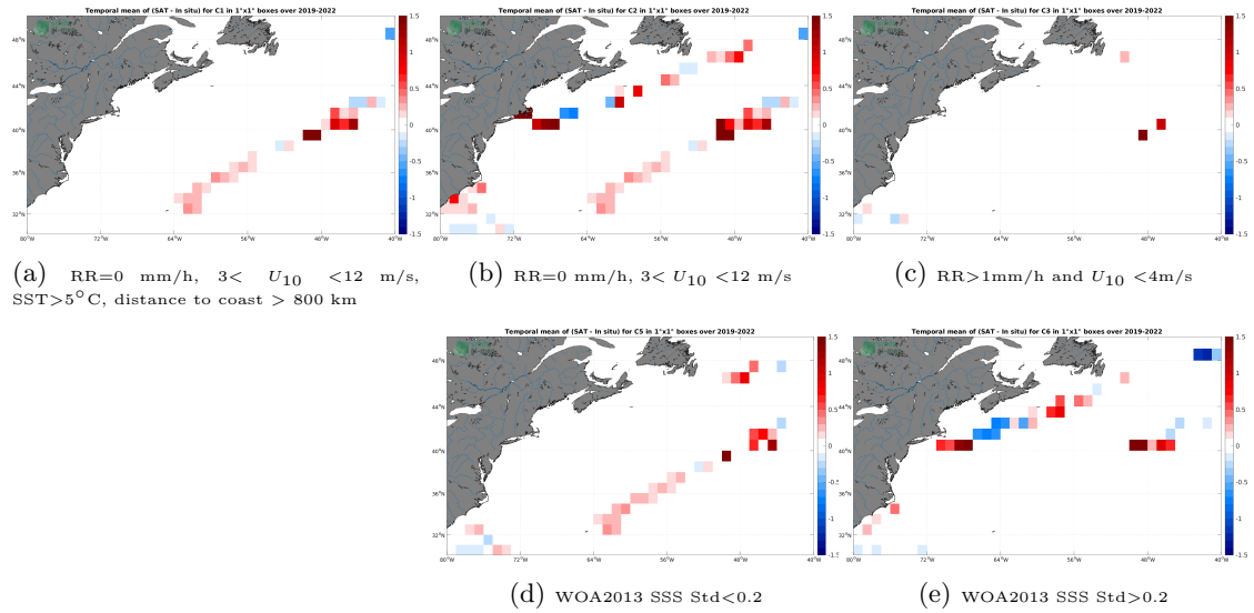
Figure 12: Temporal mean gridded over spatial boxes of size 1^\circ \times 1^\circ of \Delta SSS (SMAP SSS L4 OI v2 - 7 Days (ESR) - Sairdron) for 5 different subdatasets corresponding to:RR=0 mm/h, 3 < U_{10} < 12 m/s, SST >5^\circ C, distance to coast > 800 km (a), RR=0 mm/h, 3 < U_{10} < 12 m/s (b), RR >1 mm/h and U_{10} < 4 m/s (c), WOA2013 SSS Std <0.2 (d), WOA2013 SSS Std >0.2 (e).
