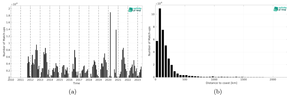
Figure 1: Number of match-ups between TSG (SAMOS) and SMAP SSS L4 OI v2 - Monthly (IPRC) SSS as a function of time (a) and as function of the distance to coast (b) over the Gulf Stream Pi-MEP region and for the full satellite product period.
