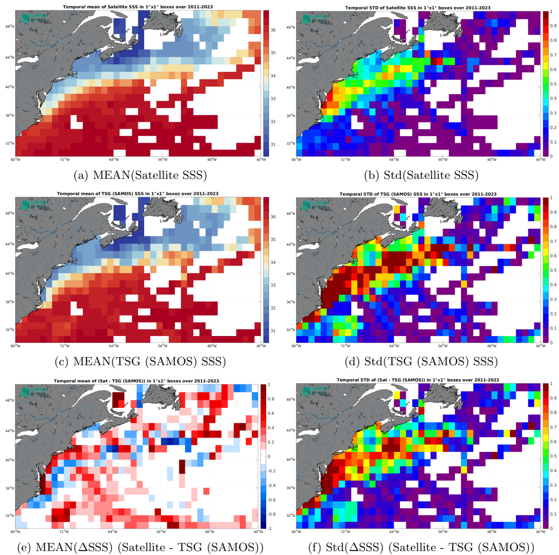
Figure 6: Temporal mean (left) and Std (right) of SSS from SMAP SSS L4 OI v2 - Monthly (IPRC) (top), TSG (SAMOS) (middle), and of \Delta SSS (Satellite - TSG (SAMOS)). Only match-up pairs are used to generate these maps.
