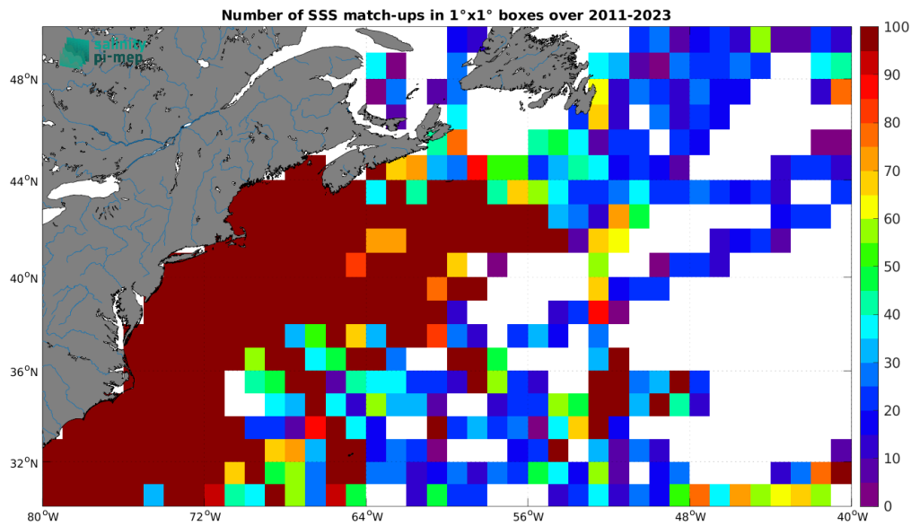
Figure 4: Number of SSS match-ups between TSG (SAMOS) SSS and the SMAP SSS L4 OI v2 - Monthly (IPRC) SSS product for the Gulf Stream Pi-MEP region over 1^\circ \times 1^\circ boxes and for the full satellite product period.
