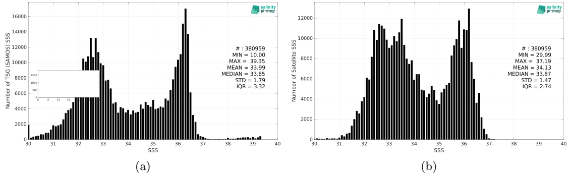
Figure 2: Histograms of SSS from TSG (SAMOS) (a) and SMAP SSS L4 OI v2 - Monthly (IPRC) (b) considering all match-up pairs per bins of 0.1 over the Gulf Stream Pi-MEP region and for the full satellite product period.
