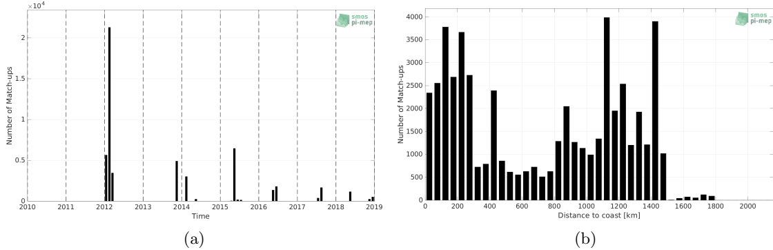
Figure 1: Number of match-ups between TSG (GOSUD-Sailing-ship) and SMAP SSS L4 OI v2 - Monthly (IPRC) SSS as a function of time (a) and as function of the distance to coast (b) over the Gulf Stream Pi-MEP region and for the full satellite product period.
