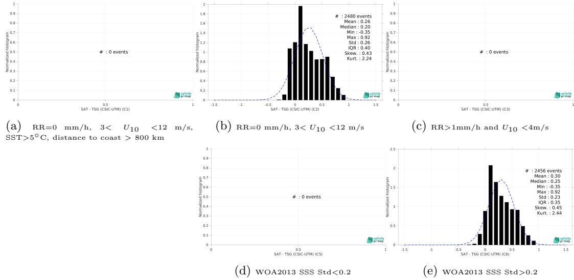
Figure 13: Normalized histogram of \Delta SSS (SMAP SSS L4 OI v2 - Monthly (IPRC) - TSG (CSIC-UTM)) for 5 different subdatasets corresponding to: RR=0 mm/h, 3 < U_{10} < 12 m/s, SST >5^{\circ} C, distance to coast > 800 km (a), RR=0 mm/h, 3 < U_{10} < 12 m/s (b), RR >1 mm/h and U_{10} < 4 m/s (c), WOA2013 SSS Std <0.2 (d), WOA2013 SSS Std >0.2 (e).
