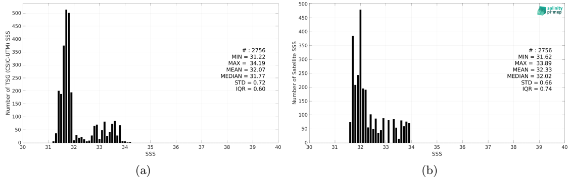
Figure 2: Histograms of SSS from TSG (CSIC-UTM) (a) and SMAP SSS L4 OI v2 - Monthly (IPRC) (b) considering all match-up pairs per bins of 0.1 over the Gulf Stream Pi-MEP region and for the full satellite product period.
