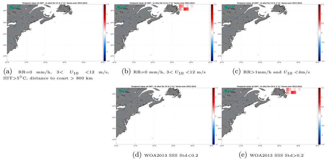
Figure 12: Temporal mean gridded over spatial boxes of size 1^{\circ}\times 1^{\circ} of \Delta\text{SSS} (SMAP SSS L4 OI v2 - Monthly (IPRC) - TSG (CSIC-UTM)) for 5 different subdatasets corresponding to:RR=0 mm/h, 3 < U_{10} < 12 m/s, SST >5^{\circ}\text{C} , distance to coast > 800 km (a), RR=0 mm/h, 3 < U_{10} < 12 m/s (b), RR >1 mm/h and U_{10} < 4 m/s (c), WOA2013 SSS Std <0.2 (d), WOA2013 SSS Std >0.2 (e).
