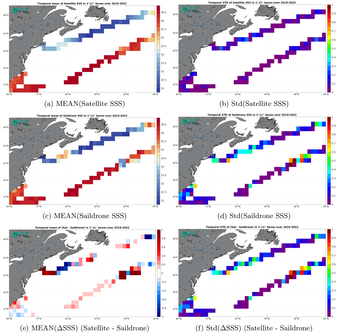
Figure 6: Temporal mean (left) and Std (right) of SSS from SMAP SSS L4 OI v2 - Monthly (IPRC) (top), Saildrone (middle), and of \Delta SSS (Satellite - Saildrone). Only match-up pairs are used to generate these maps.
