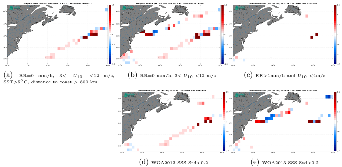
Figure 12: Temporal mean gridded over spatial boxes of size 1^\circ \times 1^\circ of \Delta SSS (SMAP SSS L4 OI v2 - Monthly (IPRC) - Saildrone) for 5 different subdatasets corresponding to:RR=0 mm/h, 3 < U_{10} < 12 m/s, SST >5^\circ C, distance to coast > 800 km (a), RR=0 mm/h, 3 < U_{10} < 12 m/s (b), RR >1 mm/h and U_{10} < 4 m/s (c), WOA2013 SSS Std <0.2 (d), WOA2013 SSS Std >0.2 (e).
