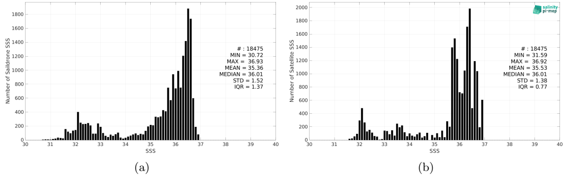
Figure 2: Histograms of SSS from SAILDRONE (a) and SMAP SSS L4 OI v2 - Monthly (IPRC) (b) considering all match-up pairs per bins of 0.1 over the Gulf Stream Pi-MEP region and for the full satellite product period.
