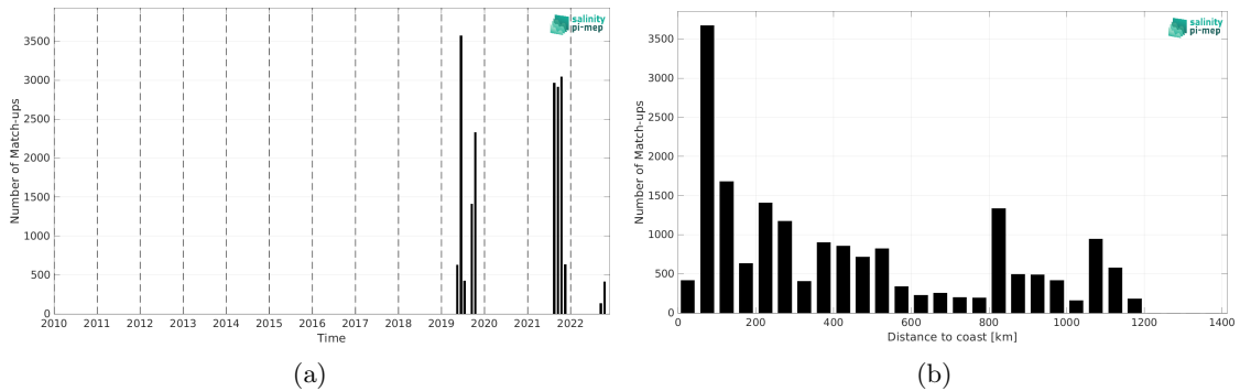
Figure 1: Number of match-ups between Saildrone and SMAP SSS L4 OI v2 - Monthly (IPRC) SSS as a function of time (a) and as function of the distance to coast (b) over the Gulf Stream Pi-MEP region and for the full satellite product period.
