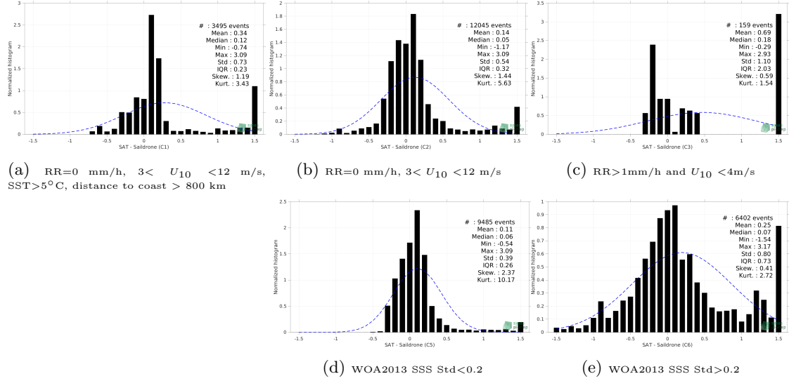
Figure 13: Normalized histogram of \Delta SSS (SMAP SSS L4 OI v2 - Monthly (IPRC) - Sairdronne) for 5 different subdatasets corresponding to: RR=0 mm/h, 3 < U_{10} < 12 m/s, SST > 5°C, distance to coast > 800 km (a), RR=0 mm/h, 3 < U_{10} < 12 m/s (b), RR > 1mm/h and U_{10} < 4 m/s (c), WOA2013 SSS Std < 0.2 (d), WOA2013 SSS Std > 0.2 (e).
