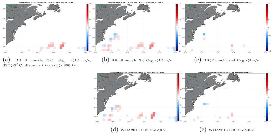
Figure 11: Temporal mean gridded over spatial boxes of size 1^{\circ}\times 1^{\circ} of \Delta\text{SSS} (SMAP SSS L4 OI v2 - Monthly (IPRC) - Surface drifters) for 5 different subdatasets corresponding to:RR=0 mm/h, 3 < U_{10} < 12 m/s, SST >5^{\circ}\text{C} , distance to coast > 800 km (a), RR=0 mm/h, 3 < U_{10} < 12 m/s (b), RR >1 mm/h and U_{10} < 4 m/s (c), WOA2013 SSS Std <0.2 (d), WOA2013 SSS Std >0.2 (e).
