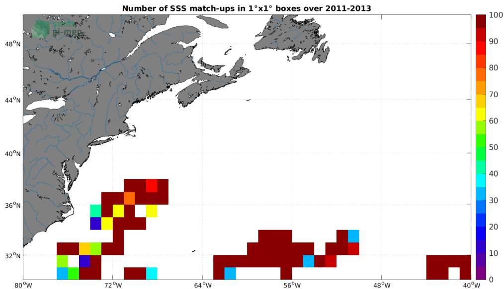
Figure 3: Number of SSS match-ups between Surface drifters SSS and the SMAP SSS L4 OI v2 - Monthly (IPRC) SSS product for the Gulf Stream Pi-MEP region over 1^\circ \times 1^\circ boxes and for the full satellite product period.
