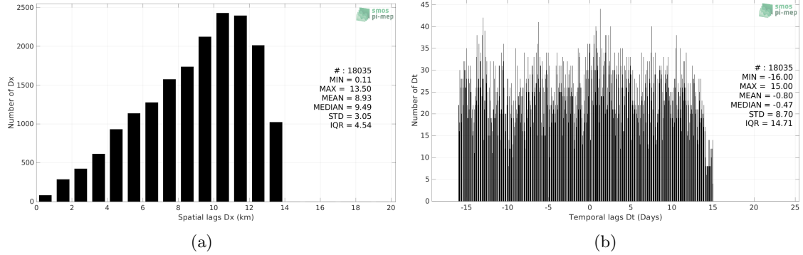
Figure 4: Histograms of the spatial (a) and temporal (b) lags between the location/time of the Surface drifters measurement and the date of the corresponding SMAP SSS L4 OI v2 - Monthly (IPRC) SSS pixel.
