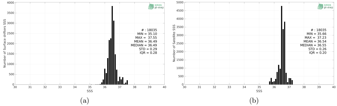
Figure 2: Histograms of SSS from Surface drifters (a) and SMAP SSS L4 OI v2 - Monthly (IPRC) (b) considering all match-up pairs per bins of 0.1 over the Gulf Stream Pi-MEP region and for the full satellite product period.
