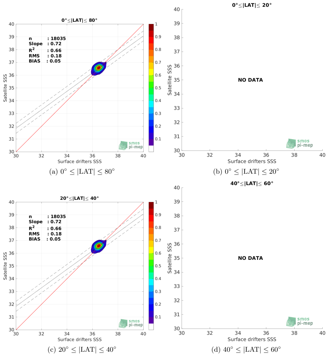
Figure 8: Contour maps of the concentration of SMAP SSS L4 OI v2 - Monthly (IPRC) SSS (y-axis) versus Surface drifters SSS (x-axis) at match-up pairs for different latitude bands. For each plot, the red line shows x=y . The black thin and dashed lines indicate a linear fit through the data cloud and the \pm 95\% confidence levels, respectively. The number match-up pairs n , the slope and R^2 coefficient of the linear fit, the root mean square (RMS) and the mean bias between satellite and in situ data are indicated for each latitude band in each plots.
