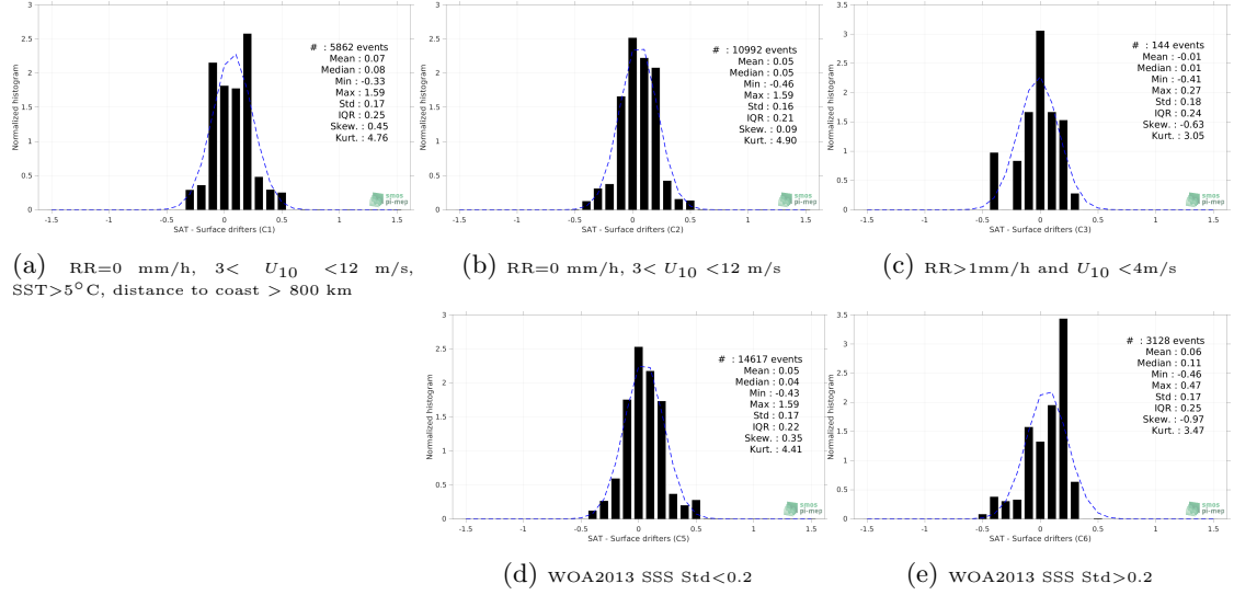
Figure 12: Normalized histogram of \Delta SSS (SMAP SSS L4 OI v2 - Monthly (IPRC) - Surface drifters) for 5 different subdatasets corresponding to: RR=0 mm/h, 3 < U_{10} < 12 m/s, SST>5°C, distance to coast > 800 km (a), RR=0 mm/h, 3 < U_{10} < 12 m/s (b), RR>1mm/h and U_{10} < 4 m/s (c), WOA2013 SSS Std<0.2 (d), WOA2013 SSS Std>0.2 (e).
