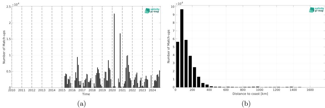
Figure 2: Number of match-ups between TSG (SAMOS) and SMAP SSS L3 v6 - 8-Day running (RSS) SSS as a function of time (a) and as function of the distance to coast (b) over the Gulf Stream Pi-MEP region and for the full satellite product period.
