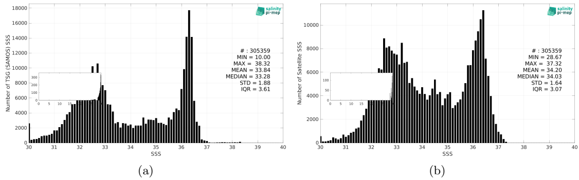
Figure 3: Histograms of SSS from TSG (SAMOS) (a) and SMAP SSS L3 v6 - 8-Day running (RSS) (b) considering all match-up pairs per bins of 0.1 over the Gulf Stream Pi-MEP region and for the full satellite product period.
