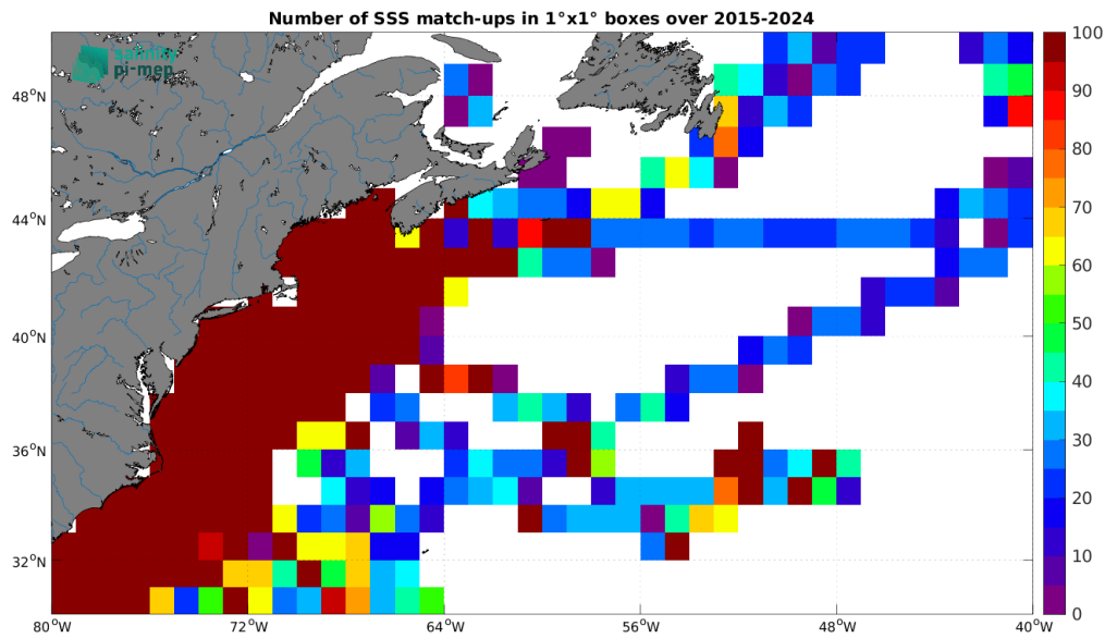
Figure 5: Number of SSS match-ups between TSG (SAMOS) SSS and the SMAP SSS L3 v6 - 8-Day running (RSS) SSS product for the Gulf Stream Pi-MEP region over 1^\circ \times 1^\circ boxes and for the full satellite product period.
