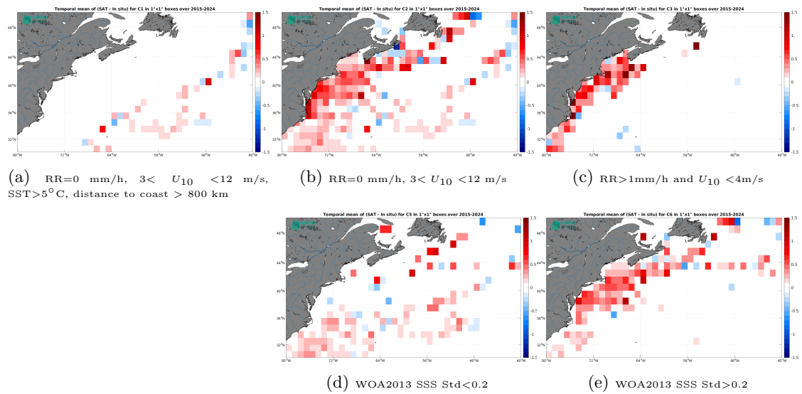
Figure 14: Temporal mean gridded over spatial boxes of size 1^\circ \times 1^\circ of \Delta SSS (SMAP SSS L3 v6 - 8-Day running (RSS) - TSG (SAMOS)) for 5 different subdatasets corresponding to:RR=0 mm/h, 3 < U_{10} < 12 m/s, SST > 5^\circ C , distance to coast > 800 km (a), RR=0 mm/h, 3 < U_{10} < 12 m/s (b), RR>1mm/h and U_{10} < 4 m/s (c), WOA2013 SSS Std<0.2 (d), WOA2013 SSS Std>0.2 (e).
