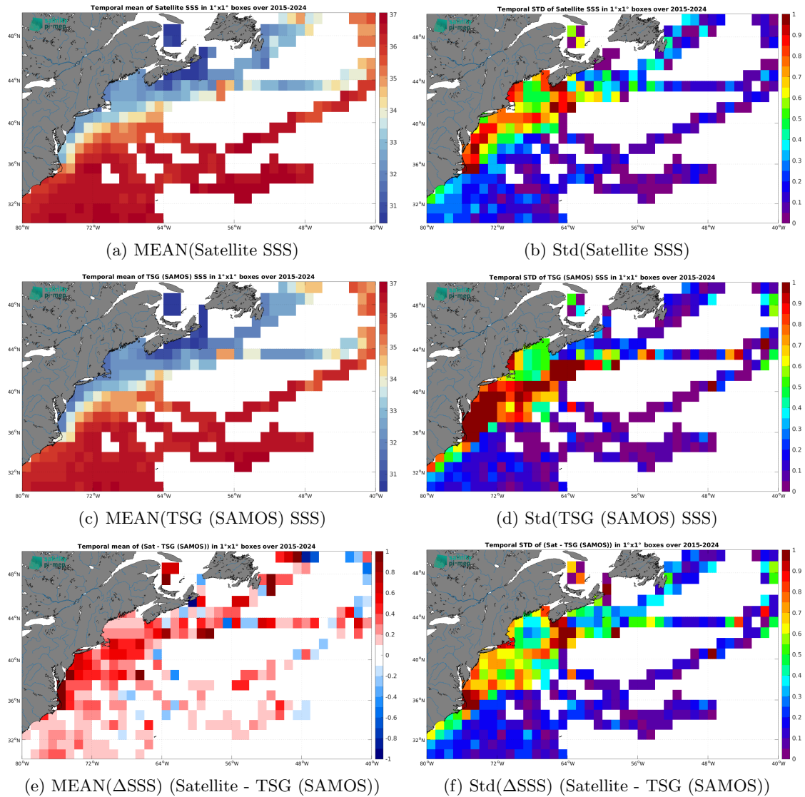
Figure 7: Temporal mean (left) and Std (right) of SSS from SMAP SSS L3 v6 - 8-Day running (RSS) (top), TSG (SAMOS) (middle), and of \Delta SSS (Satellite - TSG (SAMOS)). Only match-up pairs are used to generate these maps.
