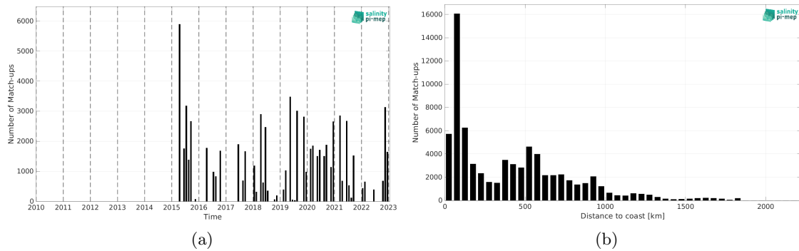
Figure 2: Number of match-ups between TSG (LEGOS-DM) and SMAP SSS L3 v6 - 8-Day running (RSS) SSS as a function of time (a) and as function of the distance to coast (b) over the Gulf Stream Pi-MEP region and for the full satellite product period.
