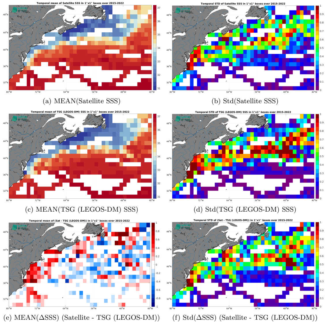
Figure 7: Temporal mean (left) and Std (right) of SSS from SMAP SSS L3 v6 - 8-Day running (RSS) (top), TSG (LEGOS-DM) (middle), and of \Delta SSS (Satellite - TSG (LEGOS-DM)). Only match-up pairs are used to generate these maps.
