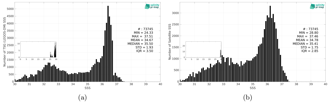
Figure 3: Histograms of SSS from TSG (LEGOS-DM) (a) and SMAP SSS L3 v6 - 8-Day running (RSS) (b) considering all match-up pairs per bins of 0.1 over the Gulf Stream Pi-MEP region and for the full satellite product period.
