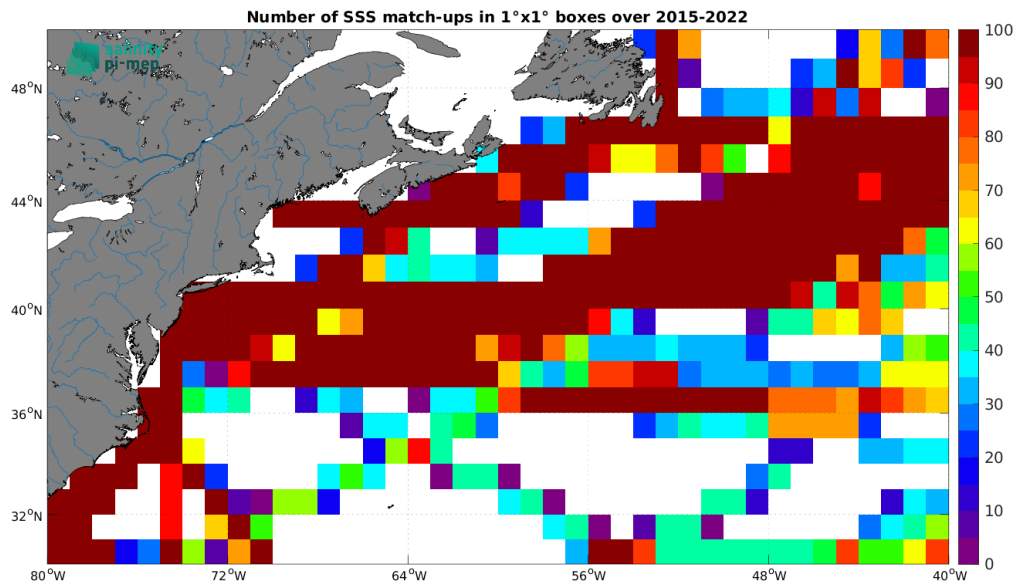
Figure 5: Number of SSS match-ups between TSG (LEGOS-DM) SSS and the SMAP SSS L3 v6 - 8-Day running (RSS) SSS product for the Gulf Stream Pi-MEP region over 1^\circ \times 1^\circ boxes and for the full satellite product period.
