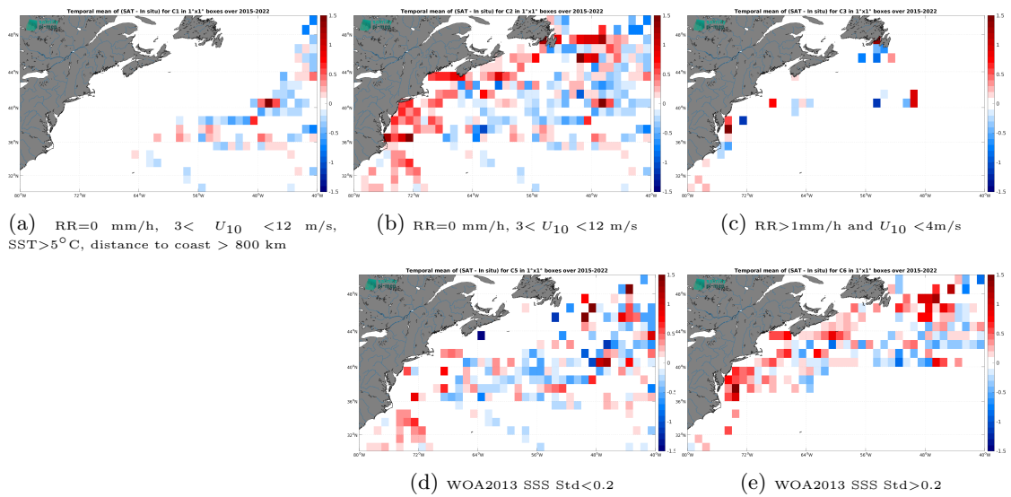
Figure 14: Temporal mean gridded over spatial boxes of size 1^\circ \times 1^\circ of \Delta SSS (SMAP SSS L3 v6 - 8-Day running (RSS) - TSG (LEGOS-DM)) for 5 different subdatasets corresponding to:RR=0 mm/h, 3 < U_{10} < 12 m/s, SST > 5°C, distance to coast > 800 km (a), RR=0 mm/h, 3 < U_{10} < 12 m/s (b), RR > 1mm/h and U_{10} < 4 m/s (c), WOA2013 SSS Std < 0.2 (d), WOA2013 SSS Std > 0.2 (e).
