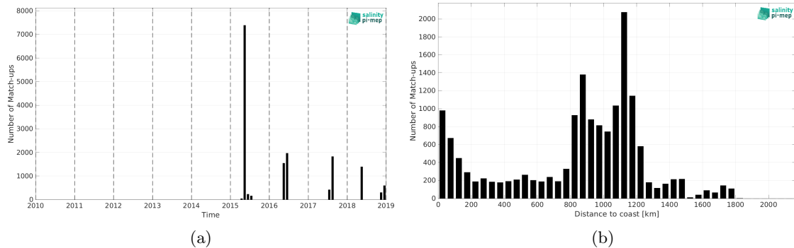
Figure 2: Number of match-ups between TSG (GOSUD-Sailing-ship) and SMAP SSS L3 v6 - 8-Day running (RSS) SSS as a function of time (a) and as function of the distance to coast (b) over the Gulf Stream Pi-MEP region and for the full satellite product period.
