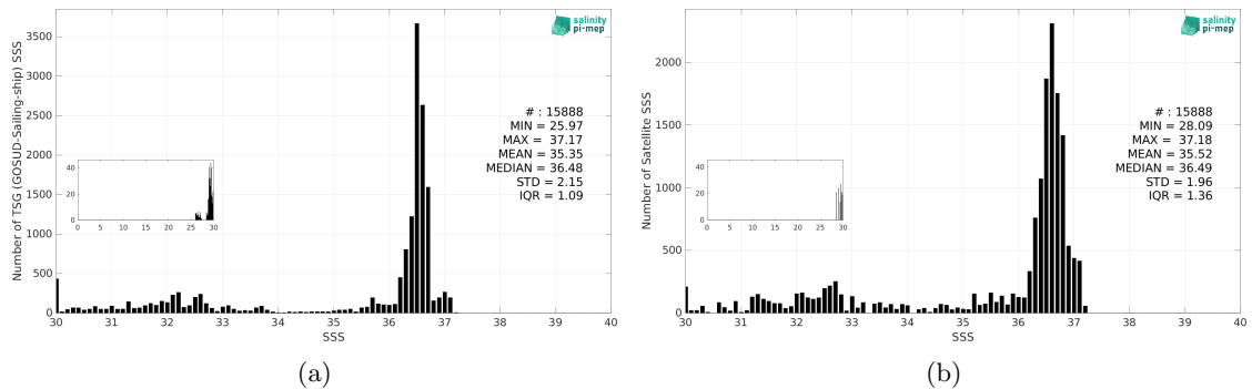
Figure 3: Histograms of SSS from TSG (GOSUD-Sailing-ship) (a) and SMAP SSS L3 v6 - 8-Day running (RSS) (b) considering all match-up pairs per bins of 0.1 over the Gulf Stream Pi-MEP region and for the full satellite product period.
