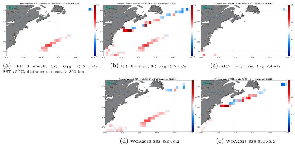
Figure 14: Temporal mean gridded over spatial boxes of size 1^\circ \times 1^\circ of \Delta SSS (SMAP SSS L3 v6 - 8-Day running (RSS) - Sairdrone) for 5 different subdatasets corresponding to:RR=0 mm/h, 3 < U_{10} < 12 m/s, SST >5^\circ C, distance to coast > 800 km (a), RR=0 mm/h, 3 < U_{10} < 12 m/s (b), RR >1 mm/h and U_{10} < 4 m/s (c), WOA2013 SSS Std <0.2 (d), WOA2013 SSS Std >0.2 (e).
