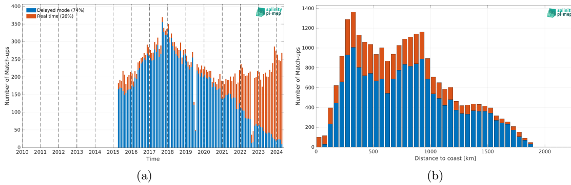
Figure 2: Number of match-ups between Argo and SMAP SSS L3 v6 - 8-Day running (RSS) SSS as a function of time (a) and as function of the distance to coast (b) over the Gulf Stream Pi-MEP region and for the full satellite product period.
