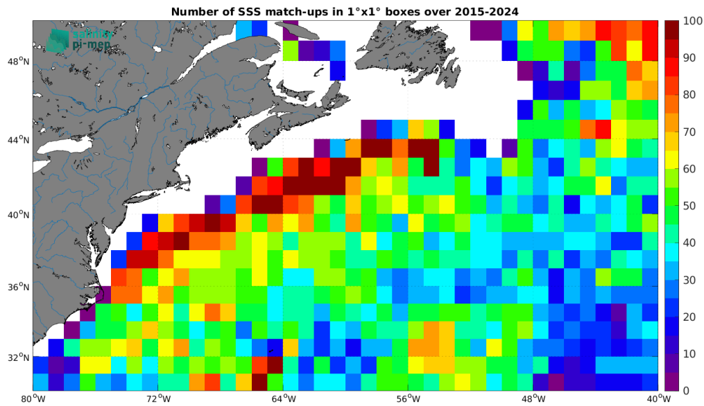
Figure 5: Number of SSS match-ups between Argo SSS and the SMAP SSS L3 v6 - 8-Day running (RSS) SSS product for the Gulf Stream Pi-MEP region over 1^\circ \times 1^\circ boxes and for the full satellite product period.
