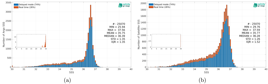
Figure 3: Histograms of SSS from Argo (a) and SMAP SSS L3 v6 - 8-Day running (RSS) (b) considering all match-up pairs per bins of 0.1 over the Gulf Stream Pi-MEP region and for the full satellite product period.
