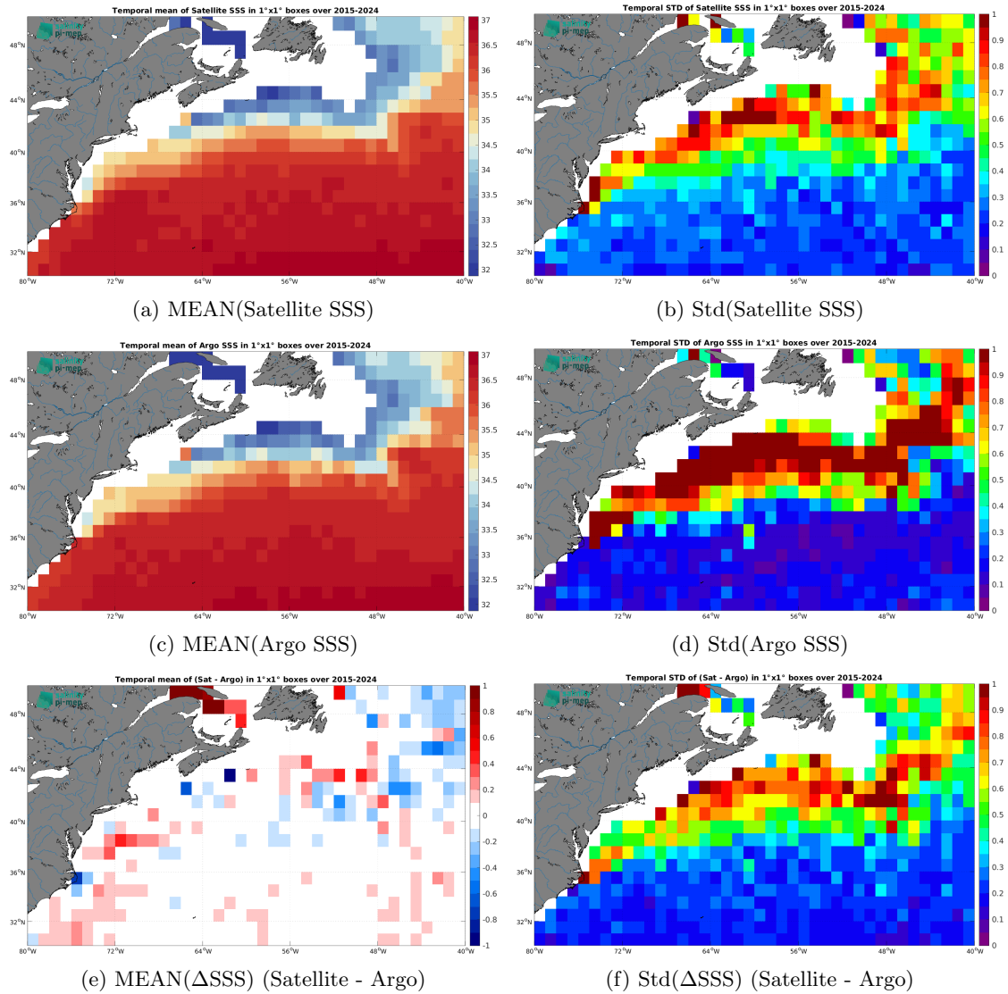
Figure 7: Temporal mean (left) and Std (right) of SSS from SMAP SSS L3 v6 - 8-Day running (RSS) (top), Argo (middle), and of \Delta SSS (Satellite - Argo). Only match-up pairs are used to generate these maps.
