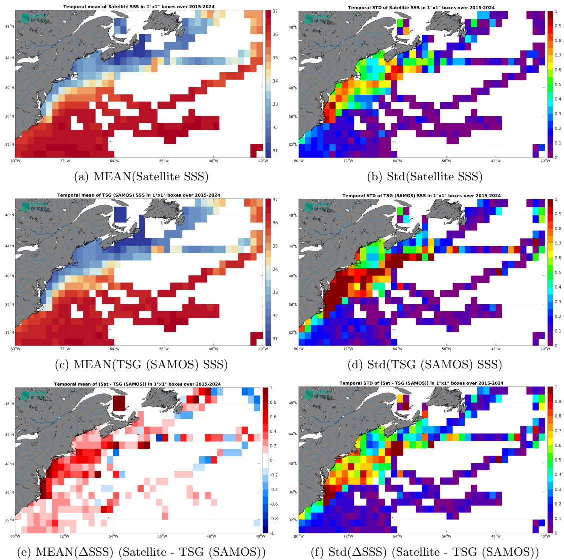
Figure 7: Temporal mean (left) and Std (right) of SSS from SMAP SSS L3 v6 - Monthly (RSS) (top), TSG (SAMOS) (middle), and of \Delta SSS (Satellite - TSG (SAMOS)). Only match-up pairs are used to generate these maps.
