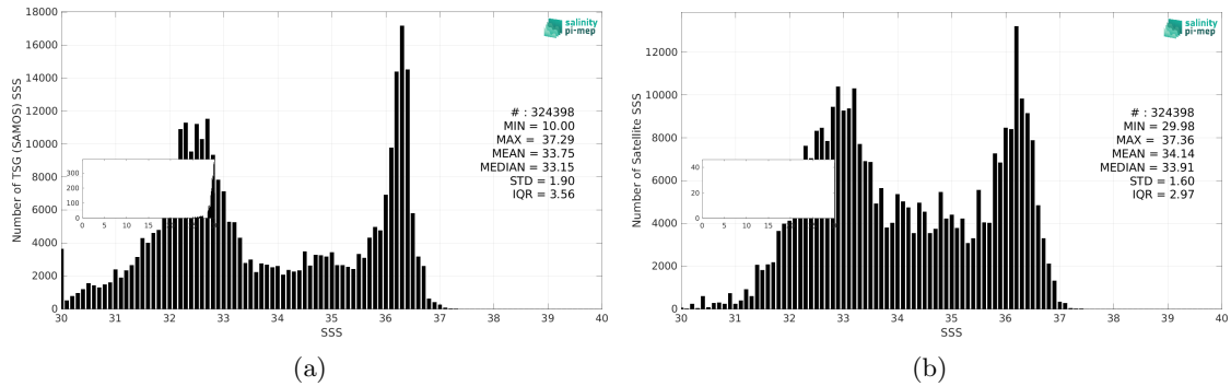
Figure 3: Histograms of SSS from TSG (SAMOS) (a) and SMAP SSS L3 v6 - Monthly (RSS) (b) considering all match-up pairs per bins of 0.1 over the Gulf Stream Pi-MEP region and for the full satellite product period.
