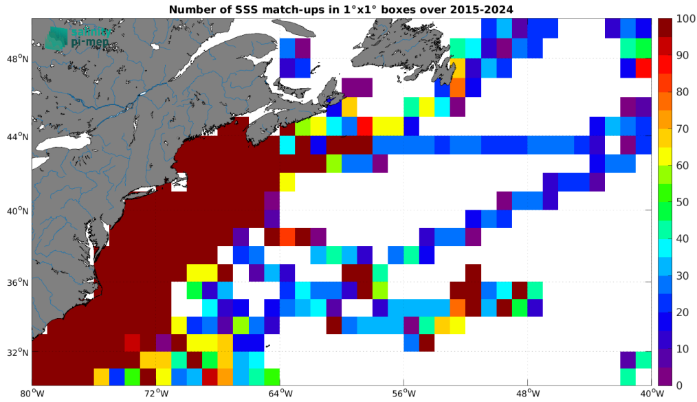
Figure 5: Number of SSS match-ups between TSG (SAMOS) SSS and the SMAP SSS L3 v6 - Monthly (RSS) SSS product for the Gulf Stream Pi-MEP region over 1^\circ \times 1^\circ boxes and for the full satellite product period.
