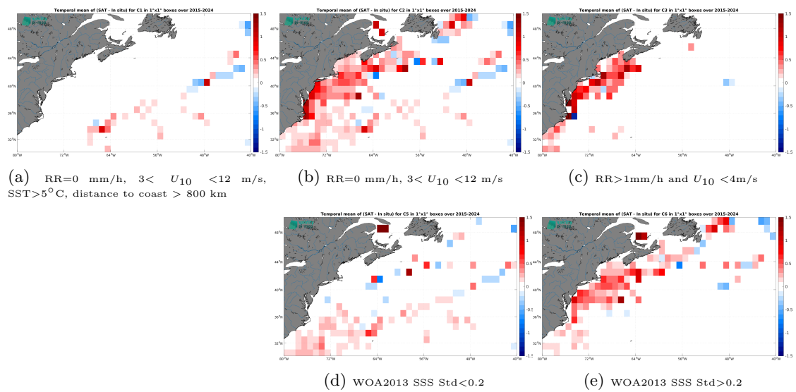
Figure 14: Temporal mean gridded over spatial boxes of size 1^\circ \times 1^\circ of \Delta SSS (SMAP SSS L3 v6 - Monthly (RSS) - TSG (SAMOS)) for 5 different subdatasets corresponding to:RR=0 mm/h, 3 < U_{10} < 12 m/s, SST>5°C, distance to coast > 800 km (a), RR=0 mm/h, 3 < U_{10} < 12 m/s (b), RR>1mm/h and U_{10} < 4 m/s (c), WOA2013 SSS Std<0.2 (d), WOA2013 SSS Std>0.2 (e).
