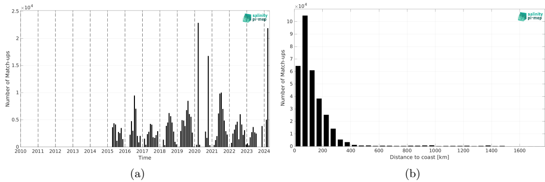
Figure 2: Number of match-ups between TSG (SAMOS) and SMAP SSS L3 v6 - Monthly (RSS) SSS as a function of time (a) and as function of the distance to coast (b) over the Gulf Stream Pi-MEP region and for the full satellite product period.
