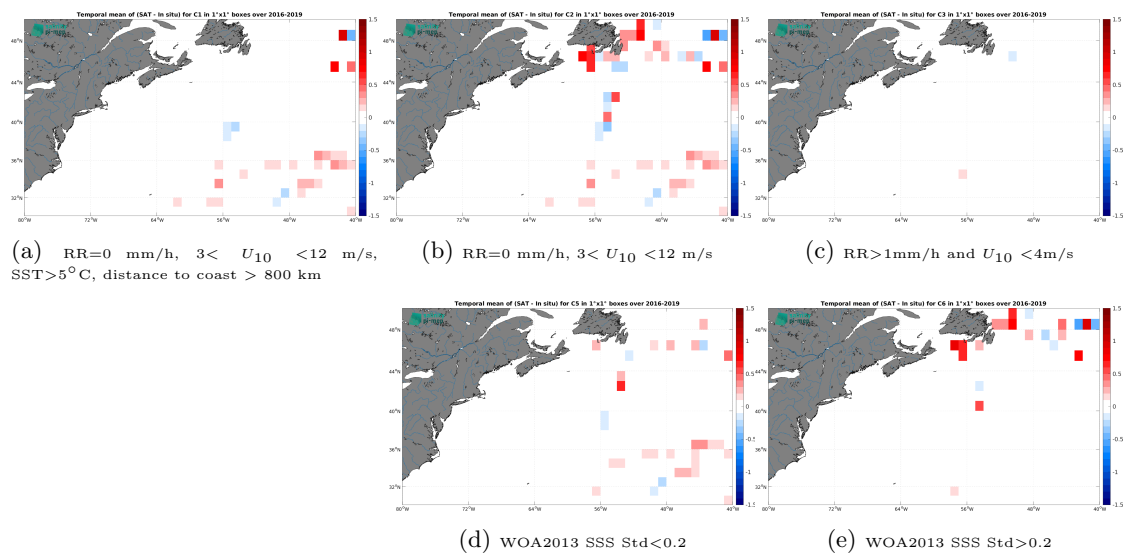
Figure 14: Temporal mean gridded over spatial boxes of size 1^\circ \times 1^\circ of \Delta SSS (SMAP SSS L3 v6 - Monthly (RSS) - TSG (GOSUD-Research-vessel)) for 5 different subdatasets corresponding to:RR=0 mm/h, 3 < U_{10} < 12 m/s, SST >5^\circ C, distance to coast > 800 km (a), RR=0 mm/h, 3 < U_{10} < 12 m/s (b), RR >1 mm/h and U_{10} < 4 m/s (c), WOA2013 SSS Std <0.2 (d), WOA2013 SSS Std >0.2 (e).
