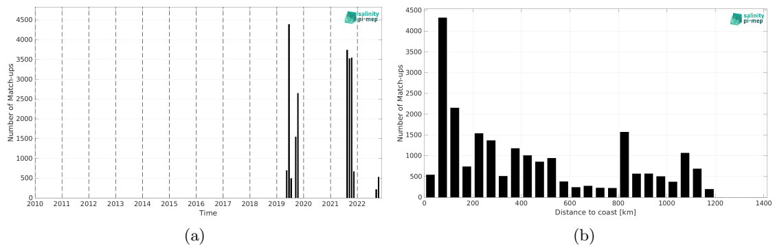
Figure 2: Number of match-ups between Saildrone and SMAP SSS L3 v6 - Monthly (RSS) SSS as a function of time (a) and as function of the distance to coast (b) over the Gulf Stream Pi-MEP region and for the full satellite product period.
