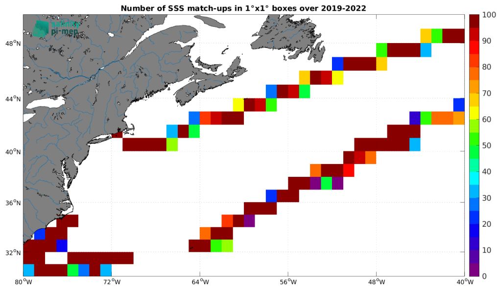
Figure 5: Number of SSS match-ups between Saildrone SSS and the SMAP SSS L3 v6 - Monthly (RSS) SSS product for the Gulf Stream Pi-MEP region over 1^\circ \times 1^\circ boxes and for the full satellite product period.
