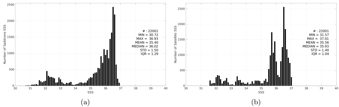
Figure 3: Histograms of SSS from Saildrone (a) and SMAP SSS L3 v6 - Monthly (RSS) (b) considering all match-up pairs per bins of 0.1 over the Gulf Stream Pi-MEP region and for the full satellite product period.
