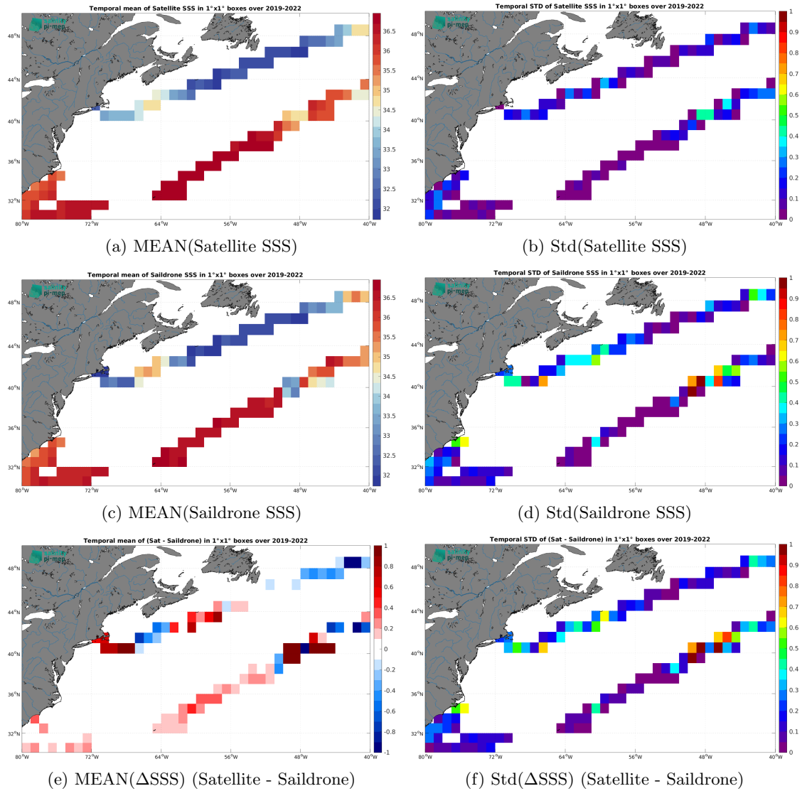
Figure 7: Temporal mean (left) and Std (right) of SSS from SMAP SSS L3 v6 - Monthly (RSS) (top), Saildrone (middle), and of \Delta SSS (Satellite - Saildrone). Only match-up pairs are used to generate these maps.
