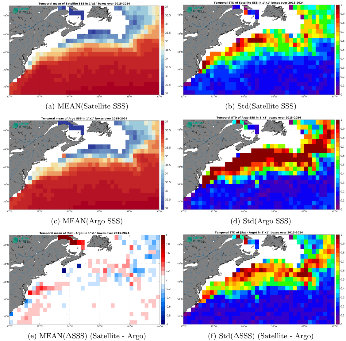
Figure 7: Temporal mean (left) and Std (right) of SSS from SMAP SSS L3 v6 - Monthly (RSS) (top), Argo (middle), and of \Delta SSS (Satellite - Argo). Only match-up pairs are used to generate these maps.
