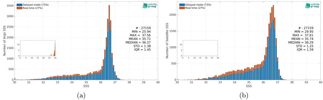
Figure 3: Histograms of SSS from Argo (a) and SMAP SSS L3 v6 - Monthly (RSS) (b) considering all match-up pairs per bins of 0.1 over the Gulf Stream Pi-MEP region and for the full satellite product period.
