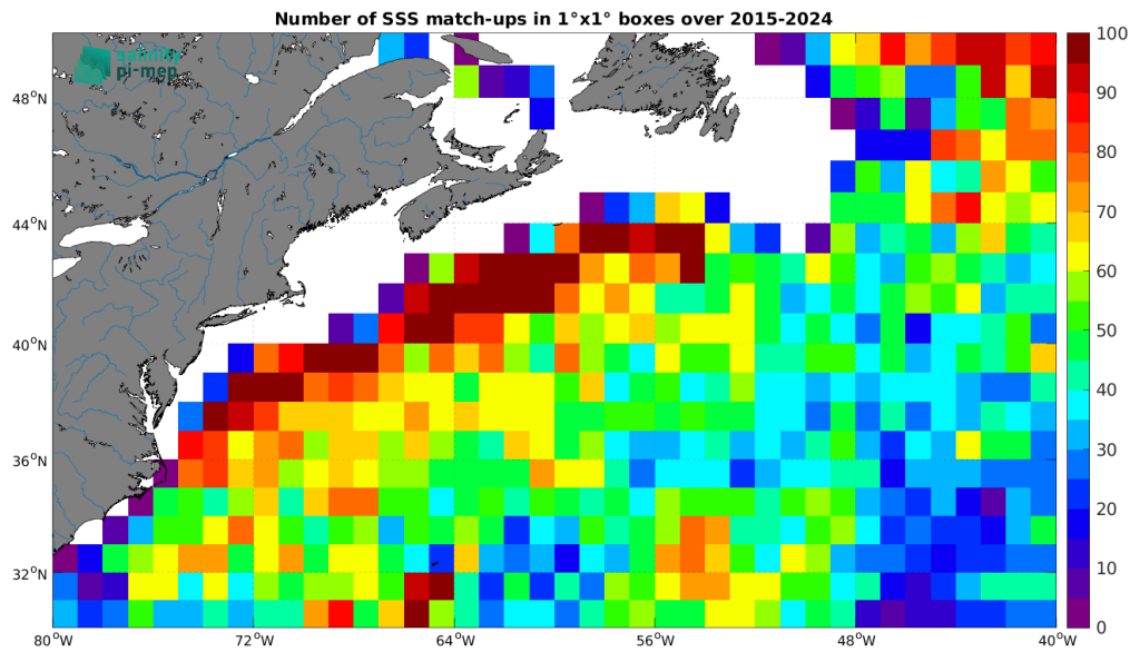
Figure 5: Number of SSS match-ups between Argo SSS and the SMAP SSS L3 v6 - Monthly (RSS) SSS product for the Gulf Stream Pi-MEP region over 1^\circ \times 1^\circ boxes and for the full satellite product period.
