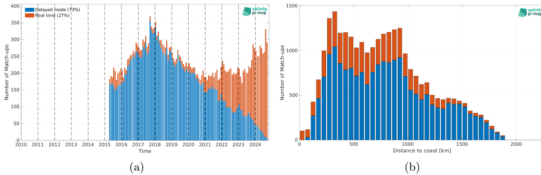
Figure 2: Number of match-ups between Argo and SMAP SSS L3 v6 - Monthly (RSS) SSS as a function of time (a) and as function of the distance to coast (b) over the Gulf Stream Pi-MEP region and for the full satellite product period.
