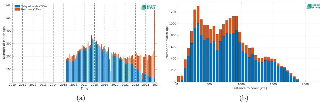
Figure 2: Number of match-ups between Argo and SMAP SSS L3 v5.3 - 8-Day running (RSS) SSS as a function of time (a) and as function of the distance to coast (b) over the Gulf Stream Pi-MEP region and for the full satellite product period.
