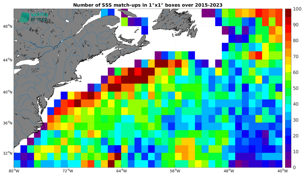
Figure 5: Number of SSS match-ups between Argo SSS and the SMAP SSS L3 v5.3 - 8-Day running (RSS) SSS product for the Gulf Stream Pi-MEP region over 1^\circ \times 1^\circ boxes and for the full satellite product period.
