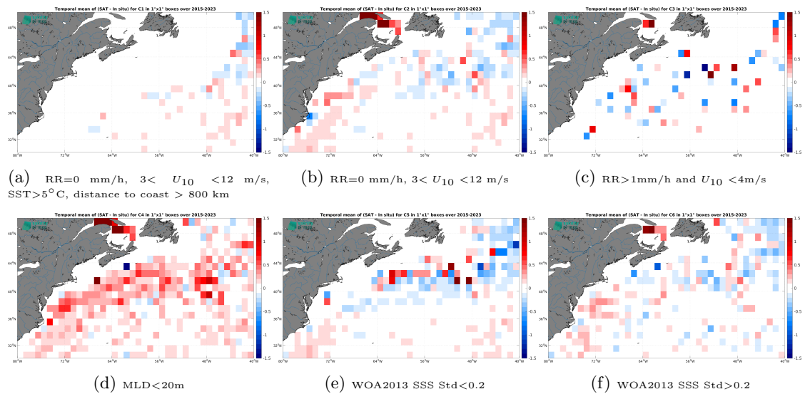
Figure 14: Temporal mean gridded over spatial boxes of size 1^\circ \times 1^\circ of \Delta SSS (SMAP SSS L3 v5.3 - 8-Day running (RSS) - Argo) for 6 different subdatasets corresponding to:RR=0 mm/h, 3 < U_{10} < 12 m/s, SST >5^\circ C, distance to coast > 800 km (a), RR=0 mm/h, 3 < U_{10} < 12 m/s (b), RR >1 mm/h and U_{10} < 4 m/s (c),MLD <20 m (d),WOA2013 SSS Std <0.2 (e),WOA2013 SSS Std >0.2 (f).
