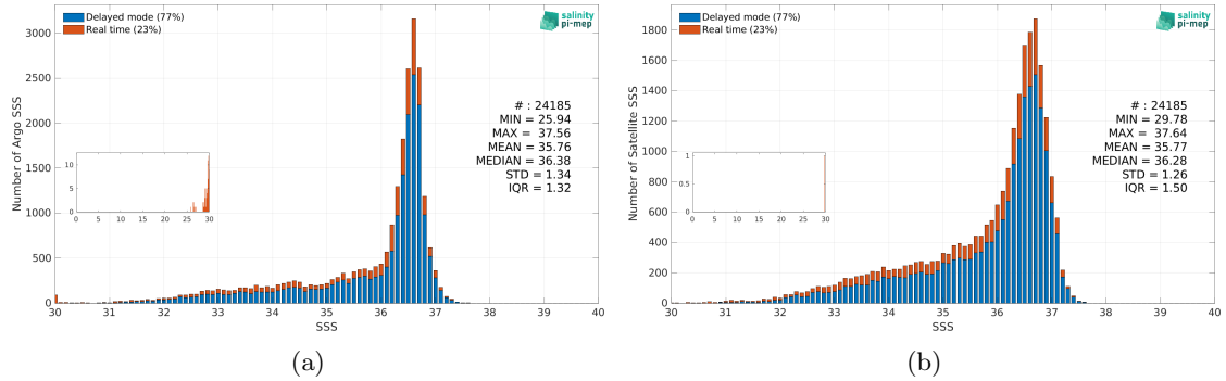
Figure 3: Histograms of SSS from Argo (a) and SMAP SSS L3 v5.3 - 8-Day running (RSS) (b) considering all match-up pairs per bins of 0.1 over the Gulf Stream Pi-MEP region and for the full satellite product period.
