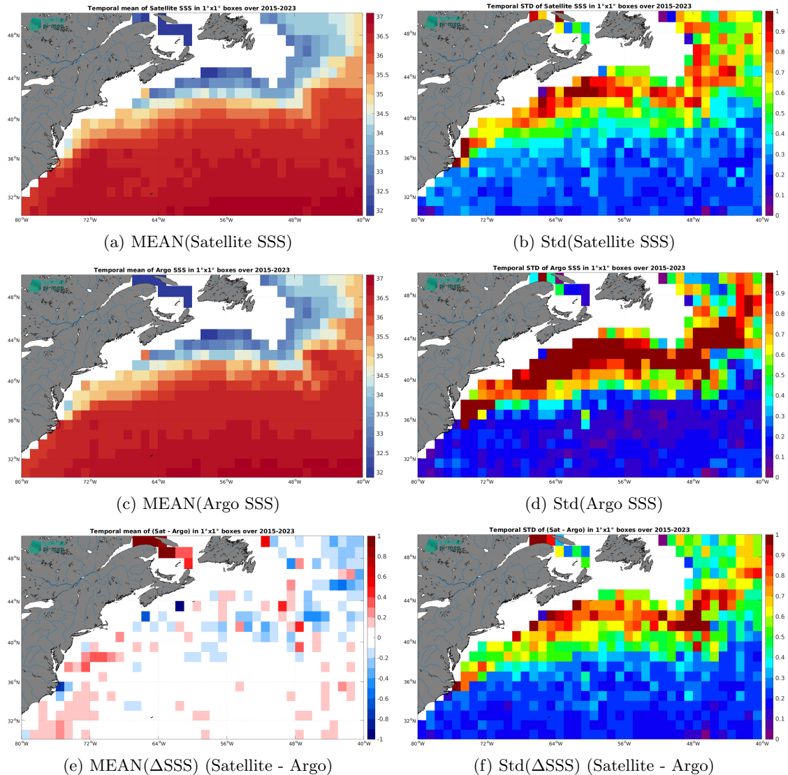
Figure 7: Temporal mean (left) and Std (right) of SSS from SMAP SSS L3 v5.3 - 8-Day running (RSS) (top), Argo (middle), and of \Delta SSS (Satellite - Argo). Only match-up pairs are used to generate these maps.
