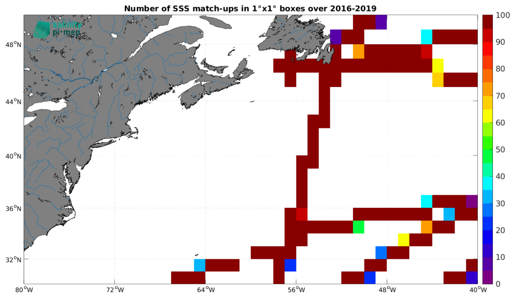
Figure 5: Number of SSS match-ups between TSG (GOSUD-Research-vessel) SSS and the SMAP SSS L3 v5.3 - Monthly (RSS) SSS product for the Gulf Stream Pi-MEP region over 1^\circ \times 1^\circ boxes and for the full satellite product period.
