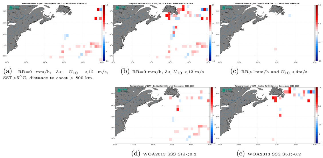
Figure 14: Temporal mean gridded over spatial boxes of size 1^\circ \times 1^\circ of \Delta SSS (SMAP SSS L3 v5.3 - Monthly (RSS) - TSG (GOSUD-Research-vessel)) for 5 different subdatasets corresponding to:RR=0 mm/h, 3 < U_{10} < 12 m/s, SST>5°C, distance to coast > 800 km (a), RR=0 mm/h, 3 < U_{10} < 12 m/s (b), RR>1mm/h and U_{10} < 4 m/s (c), WOA2013 SSS Std<0.2 (d), WOA2013 SSS Std>0.2 (e).
