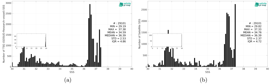
Figure 3: Histograms of SSS from TSG (GOSUD-Research-vessel) (a) and SMAP SSS L3 v5.3 - Monthly (RSS) (b) considering all match-up pairs per bins of 0.1 over the Gulf Stream Pi-MEP region and for the full satellite product period.
