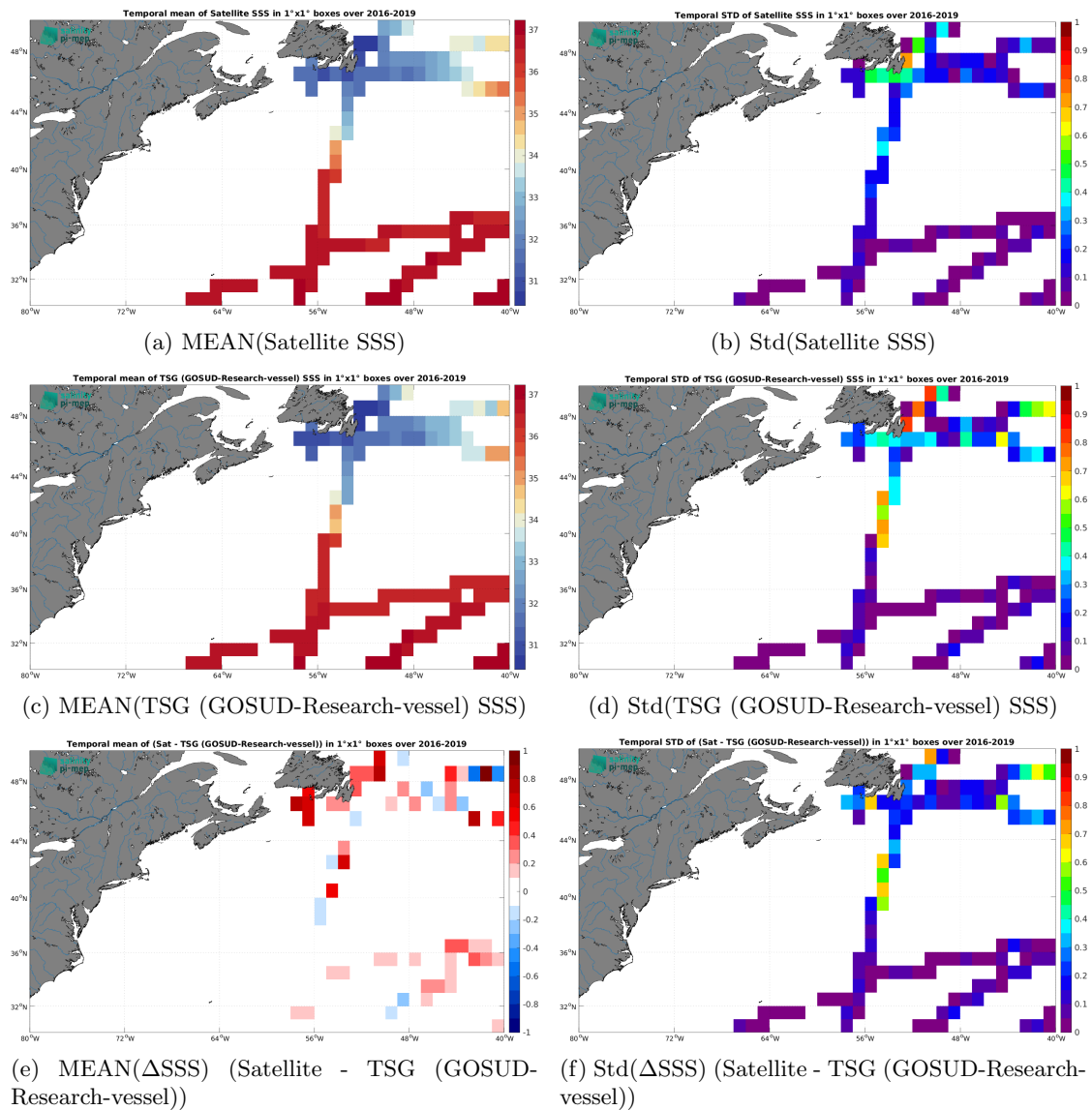
Figure 7: Temporal mean (left) and Std (right) of SSS from SMAP SSS L3 v5.3 - Monthly (RSS) (top), TSG (GOSUD-Research-vessel) (middle), and of \Delta SSS (Satellite - TSG (GOSUD-Research-vessel)). Only match-up pairs are used to generate these maps.
