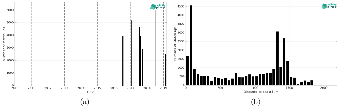
Figure 2: Number of match-ups between TSG (GOSUD-Research-vessel) and SMAP SSS L3 v5.3 - Monthly (RSS) SSS as a function of time (a) and as function of the distance to coast (b) over the Gulf Stream Pi-MEP region and for the full satellite product period.
