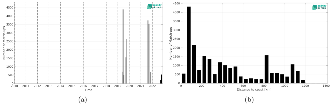
Figure 2: Number of match-ups between Saildrone and SMAP SSS L3 v5.3 - Monthly (RSS) SSS as a function of time (a) and as function of the distance to coast (b) over the Gulf Stream Pi-MEP region and for the full satellite product period.
