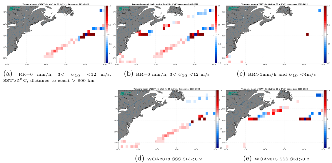
Figure 14: Temporal mean gridded over spatial boxes of size 1^\circ \times 1^\circ of \Delta SSS (SMAP SSS L3 v5.3 - Monthly (RSS) - Sairdrone) for 5 different subdatasets corresponding to:RR=0 mm/h, 3 < U_{10} < 12 m/s, SST>5°C, distance to coast > 800 km (a), RR=0 mm/h, 3 < U_{10} < 12 m/s (b), RR>1mm/h and U_{10} < 4 m/s (c), WOA2013 SSS Std<0.2 (d), WOA2013 SSS Std>0.2 (e).
