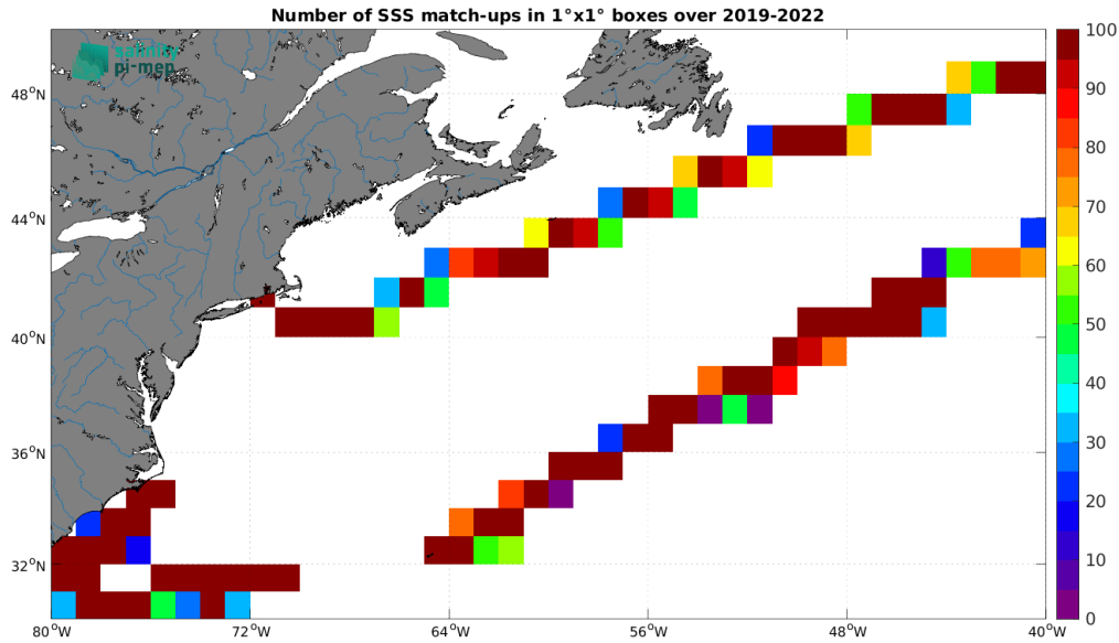
Figure 5: Number of SSS match-ups between Saildrone SSS and the SMAP SSS L3 v5.3 - Monthly (RSS) SSS product for the Gulf Stream Pi-MEP region over 1^\circ \times 1^\circ boxes and for the full satellite product period.
