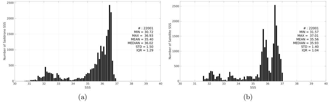
Figure 3: Histograms of SSS from Saildrone (a) and SMAP SSS L3 v5.3 - Monthly (RSS) (b) considering all match-up pairs per bins of 0.1 over the Gulf Stream Pi-MEP region and for the full satellite product period.
