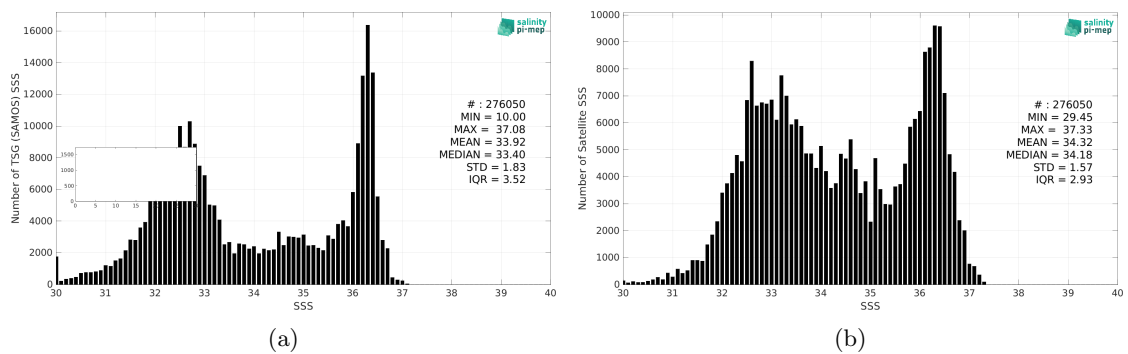
Figure 2: Histograms of SSS from TSG (SAMOS) (a) and SMAP SSS L3 v5 - 8-Day running (RSS) (b) considering all match-up pairs per bins of 0.1 over the Gulf Stream Pi-MEP region and for the full satellite product period.
