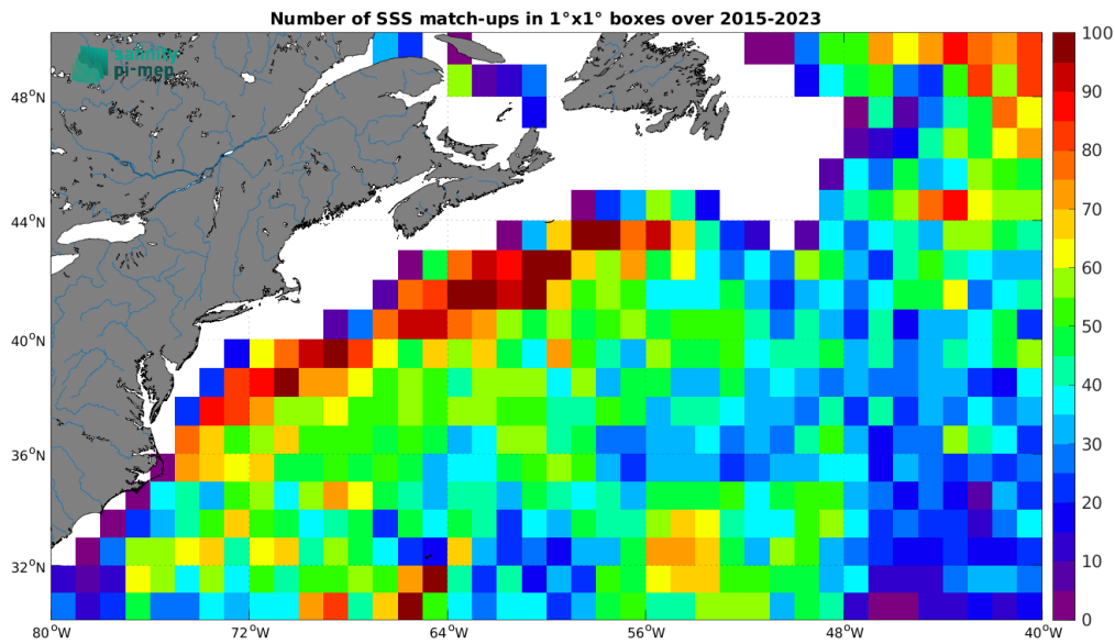
Figure 4: Number of SSS match-ups between Argo SSS and the SMAP SSS L3 v5 - 8-Day running (RSS) SSS product for the Gulf Stream Pi-MEP region over 1^\circ \times 1^\circ boxes and for the full satellite product period.
