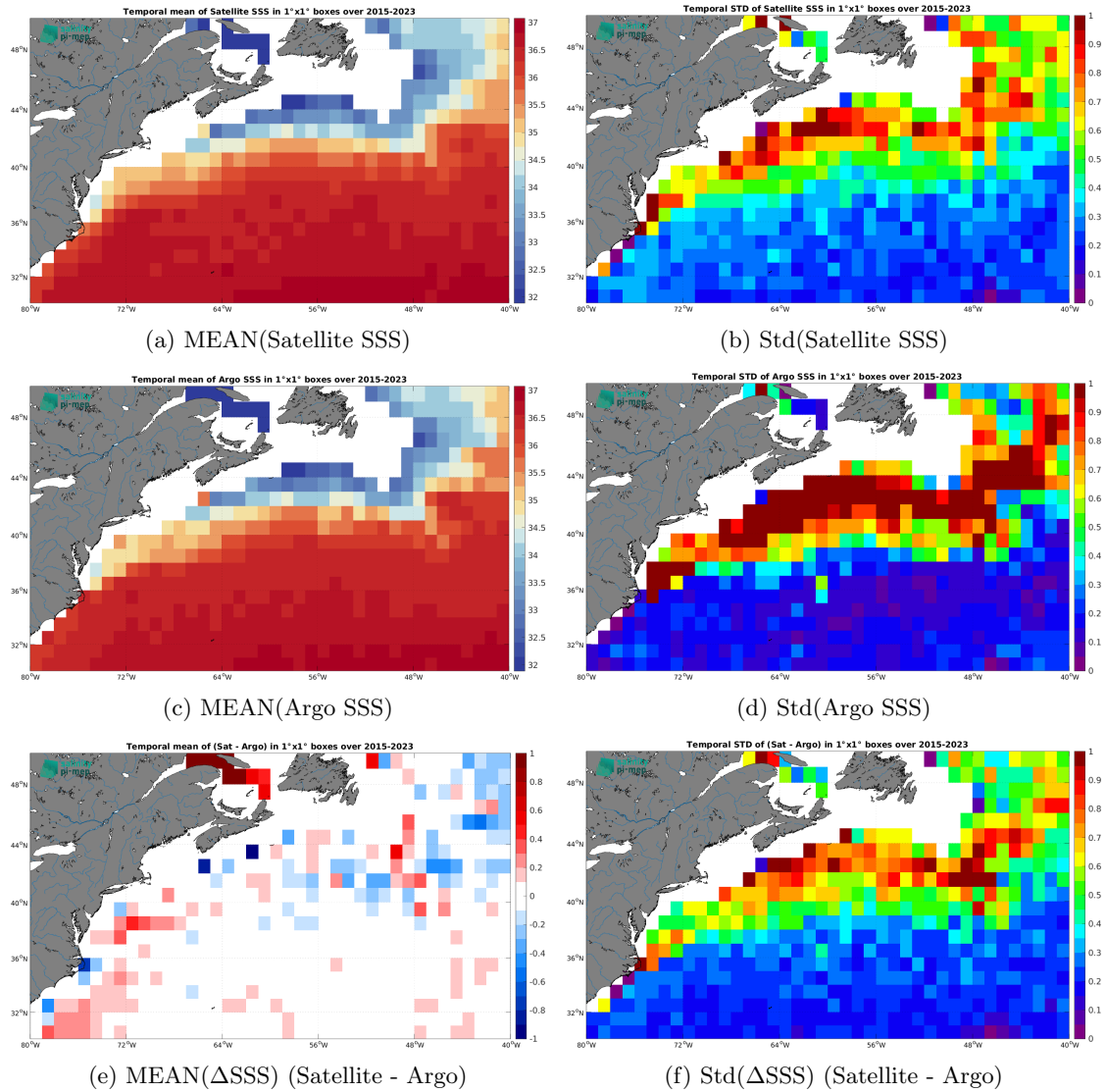
Figure 6: Temporal mean (left) and Std (right) of SSS from SMAP SSS L3 v5 - 8-Day running (RSS) (top), Argo (middle), and of \Delta SSS (Satellite - Argo). Only match-up pairs are used to generate these maps.
