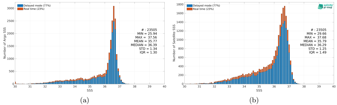
Figure 2: Histograms of SSS from Argo (a) and SMAP SSS L3 v5 - 8-Day running (RSS) (b) considering all match-up pairs per bins of 0.1 over the Gulf Stream Pi-MEP region and for the full satellite product period.
