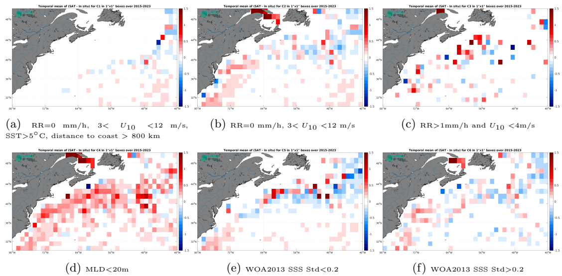
Figure 12: Temporal mean gridded over spatial boxes of size 1^\circ \times 1^\circ of \Delta SSS (SMAP SSS L3 v5 - 8-Day running (RSS) - Argo) for 6 different subdatasets corresponding to:RR=0 mm/h, 3 < U_{10} < 12 m/s, SST >5^\circ C, distance to coast > 800 km (a), RR=0 mm/h, 3 < U_{10} < 12 m/s (b), RR >1 mm/h and U_{10} < 4 m/s (c),MLD <20 m (d),WOA2013 SSS Std <0.2 (e),WOA2013 SSS Std >0.2 (f).
