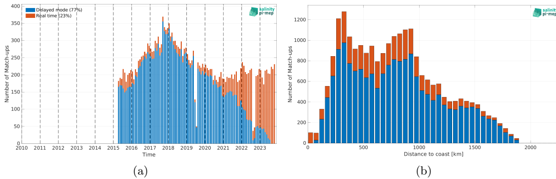
Figure 1: Number of match-ups between Argo and SMAP SSS L3 v5 - 8-Day running (RSS) SSS as a function of time (a) and as function of the distance to coast (b) over the Gulf Stream Pi-MEP region and for the full satellite product period.
