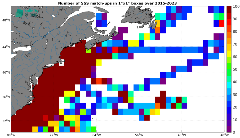
Figure 4: Number of SSS match-ups between TSG (SAMOS) SSS and the SMAP SSS L3 v5 - Monthly (RSS) SSS product for the Gulf Stream Pi-MEP region over 1^{\circ} \times 1^{\circ} boxes and for the full satellite product period.
