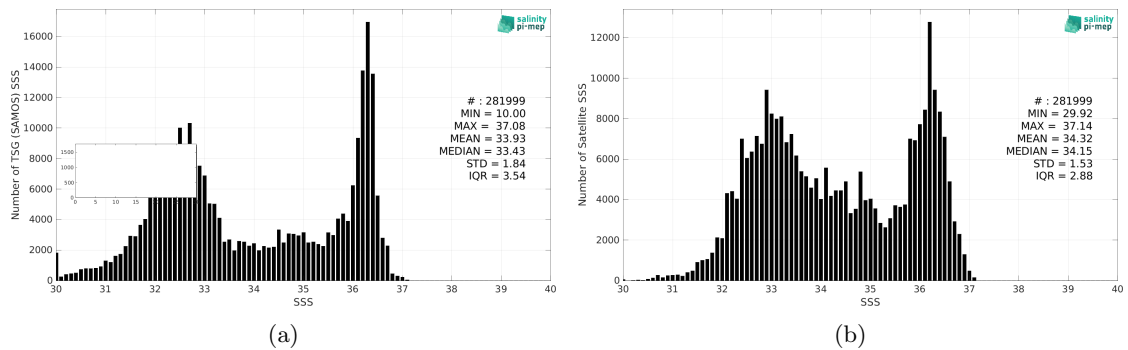
Figure 2: Histograms of SSS from TSG (SAMOS) (a) and SMAP SSS L3 v5 - Monthly (RSS) (b) considering all match-up pairs per bins of 0.1 over the Gulf Stream Pi-MEP region and for the full satellite product period.
