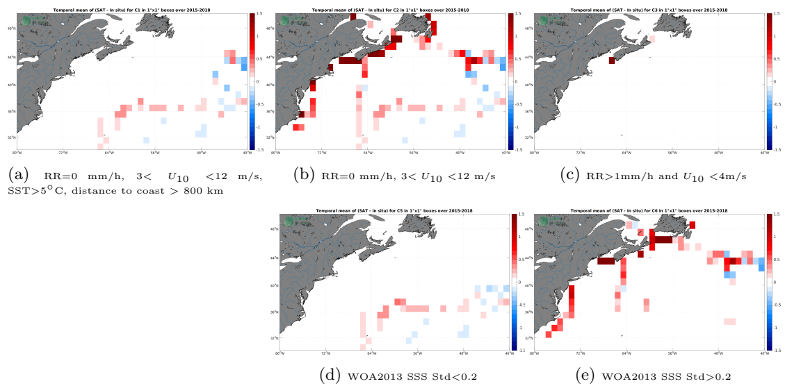
Figure 12: Temporal mean gridded over spatial boxes of size 1^\circ \times 1^\circ of \Delta SSS (SMAP SSS L3 v5 - Monthly (RSS) - TSG (GOSUD-Sailing-ship)) for 5 different subdatasets corresponding to:RR=0 mm/h, 3 < U_{10} < 12 m/s, SST>5°C, distance to coast > 800 km (a), RR=0 mm/h, 3 < U_{10} < 12 m/s (b), RR>1mm/h and U_{10} < 4 m/s (c), WOA2013 SSS Std<0.2 (d), WOA2013 SSS Std>0.2 (e).
