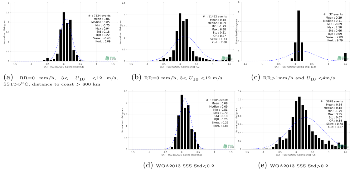
Figure 13: Normalized histogram of \Delta SSS (SMAP SSS L3 v5 - Monthly (RSS) - TSG (GOSUD-Sailing-ship)) for 5 different subdatasets corresponding to: RR=0 mm/h, 3 < U_{10} < 12 m/s, SST > 5^\circ\text{C} , distance to coast > 800 km (a), RR=0 mm/h, 3 < U_{10} < 12 m/s (b), RR > 1\text{mm/h} and U_{10} < 4\text{m/s} (c), WOA2013 SSS Std < 0.2 (d), WOA2013 SSS Std > 0.2 (e).
