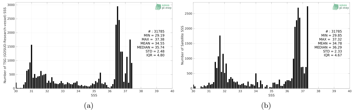
Figure 2: Histograms of SSS from TSG (GOSUD-Research-vessel) (a) and SMAP SSS L3 v5 - Monthly (RSS) (b) considering all match-up pairs per bins of 0.1 over the Gulf Stream Pi-MEP region and for the full satellite product period.
