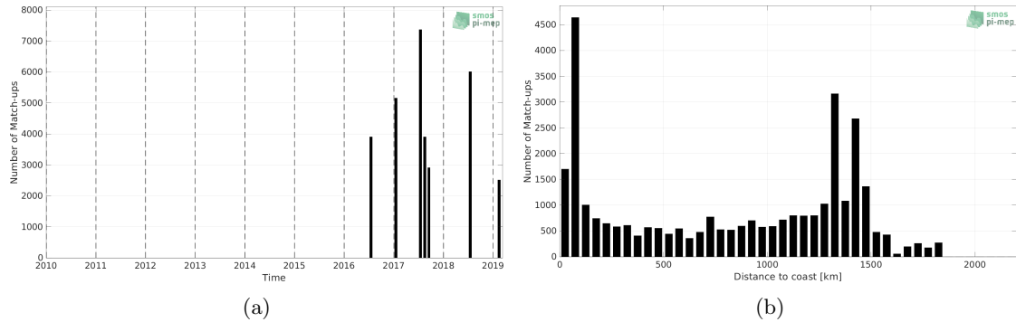
Figure 1: Number of match-ups between TSG (GOSUD-Research-vessel) and SMAP SSS L3 v5 - Monthly (RSS) SSS as a function of time (a) and as function of the distance to coast (b) over the Gulf Stream Pi-MEP region and for the full satellite product period.
