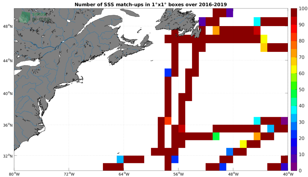
Figure 4: Number of SSS match-ups between TSG (GOSUD-Research-vessel) SSS and the SMAP SSS L3 v5 - Monthly (RSS) SSS product for the Gulf Stream Pi-MEP region over 1^\circ \times 1^\circ boxes and for the full satellite product period.
