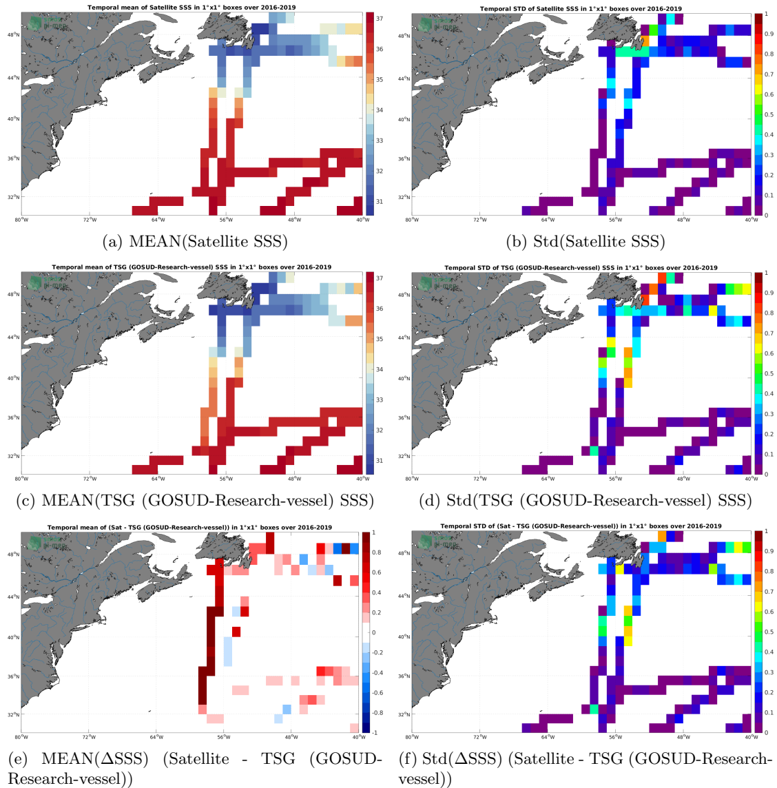
Figure 6: Temporal mean (left) and Std (right) of SSS from SMAP SSS L3 v5 - Monthly (RSS) (top), TSG (GOSUD-Research-vessel) (middle), and of \Delta SSS (Satellite - TSG (GOSUD-Research-vessel)). Only match-up pairs are used to generate these maps.
