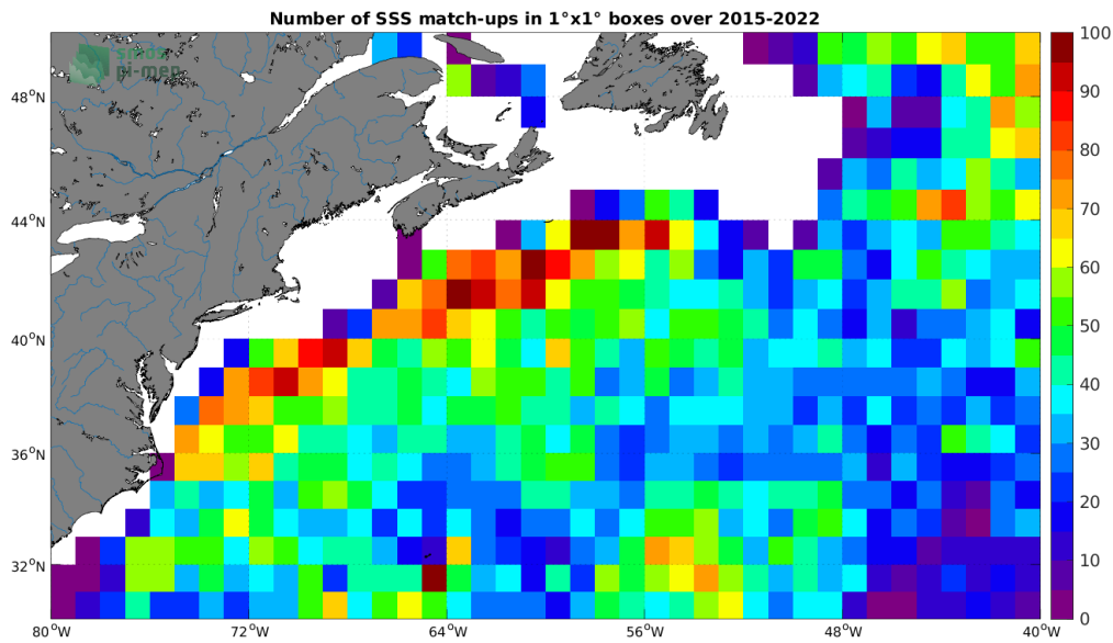
Figure 4: Number of SSS match-ups between Argo SSS and the SMAP SSS L3 v5 - Monthly (RSS) SSS product for the Gulf Stream Pi-MEP region over 1^\circ \times 1^\circ boxes and for the full satellite product period.
