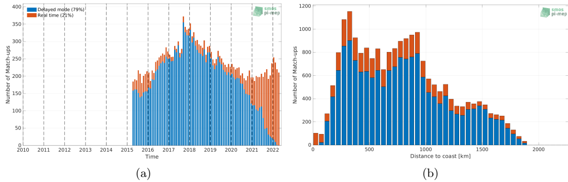
Figure 1: Number of match-ups between Argo and SMAP SSS L3 v5 - Monthly (RSS) SSS as a function of time (a) and as function of the distance to coast (b) over the Gulf Stream Pi-MEP region and for the full satellite product period.
