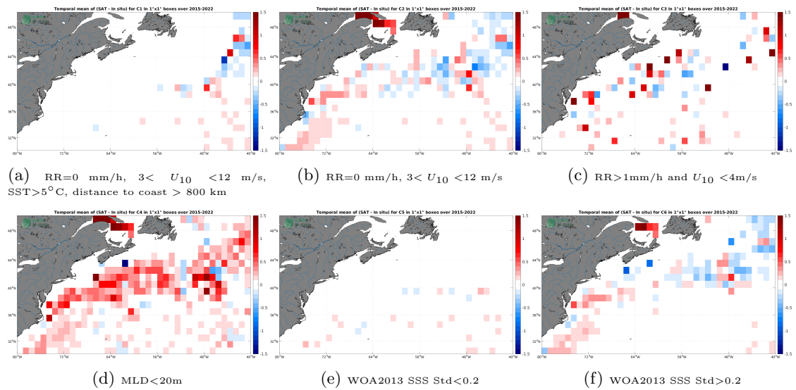
Figure 12: Temporal mean gridded over spatial boxes of size 1^\circ \times 1^\circ of \Delta SSS (SMAP SSS L3 v5 - Monthly (RSS) - Argo) for 6 different subdatasets corresponding to:RR=0 mm/h, 3 < U_{10} < 12 m/s, SST > 5^\circ\text{C} , distance to coast > 800 km (a), RR=0 mm/h, 3 < U_{10} < 12 m/s (b), RR > 1 mm/h and U_{10} < 4 m/s (c),MLD < 20 m (d),WOA2013 SSS Std < 0.2 (e),WOA2013 SSS Std > 0.2 (f).
