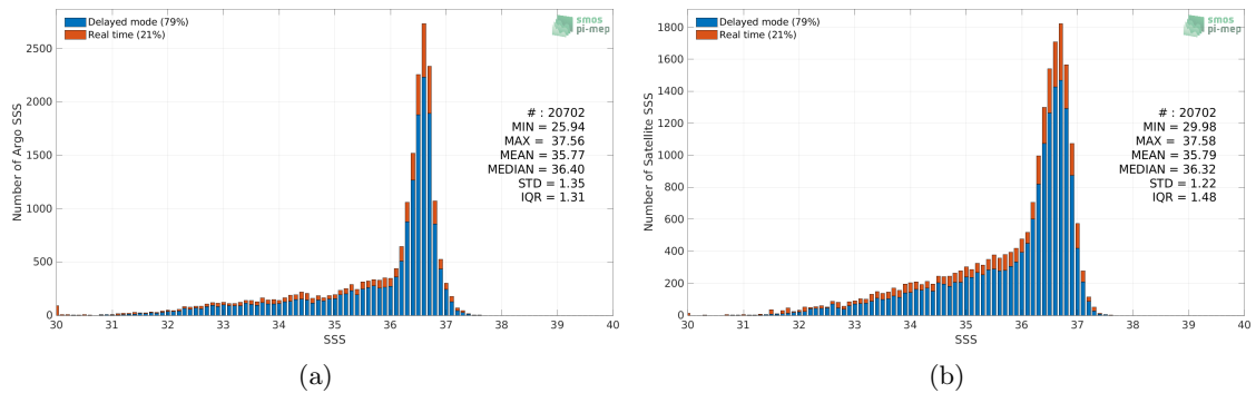
Figure 2: Histograms of SSS from Argo (a) and SMAP SSS L3 v5 - Monthly (RSS) (b) considering all match-up pairs per bins of 0.1 over the Gulf Stream Pi-MEP region and for the full satellite product period.
